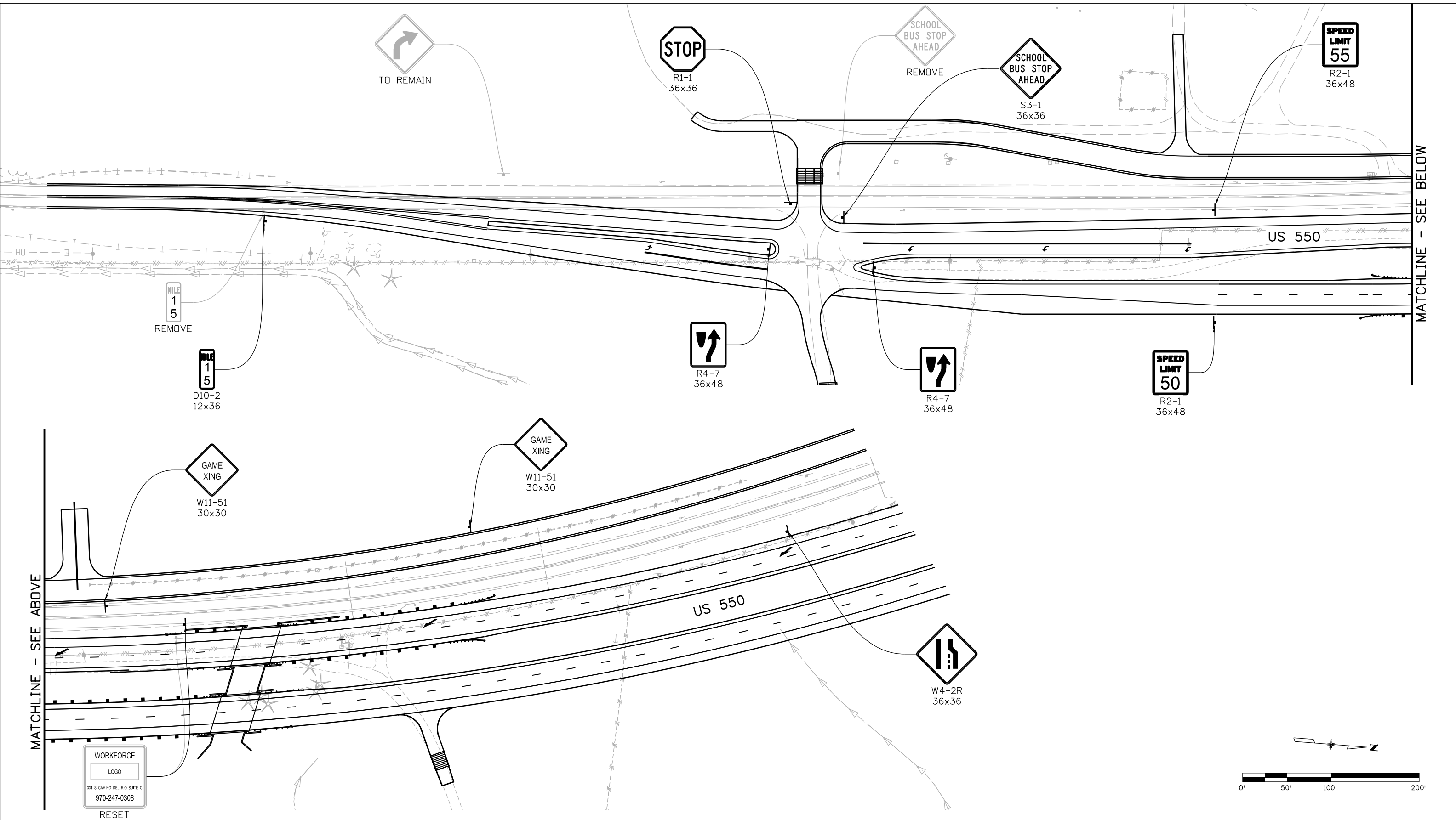
BASIC CONFIGURATION TRANSITION DETAIL SIGNING AND STRIPING NHPP 5501-029, 22420 JUNE 10, 2019
