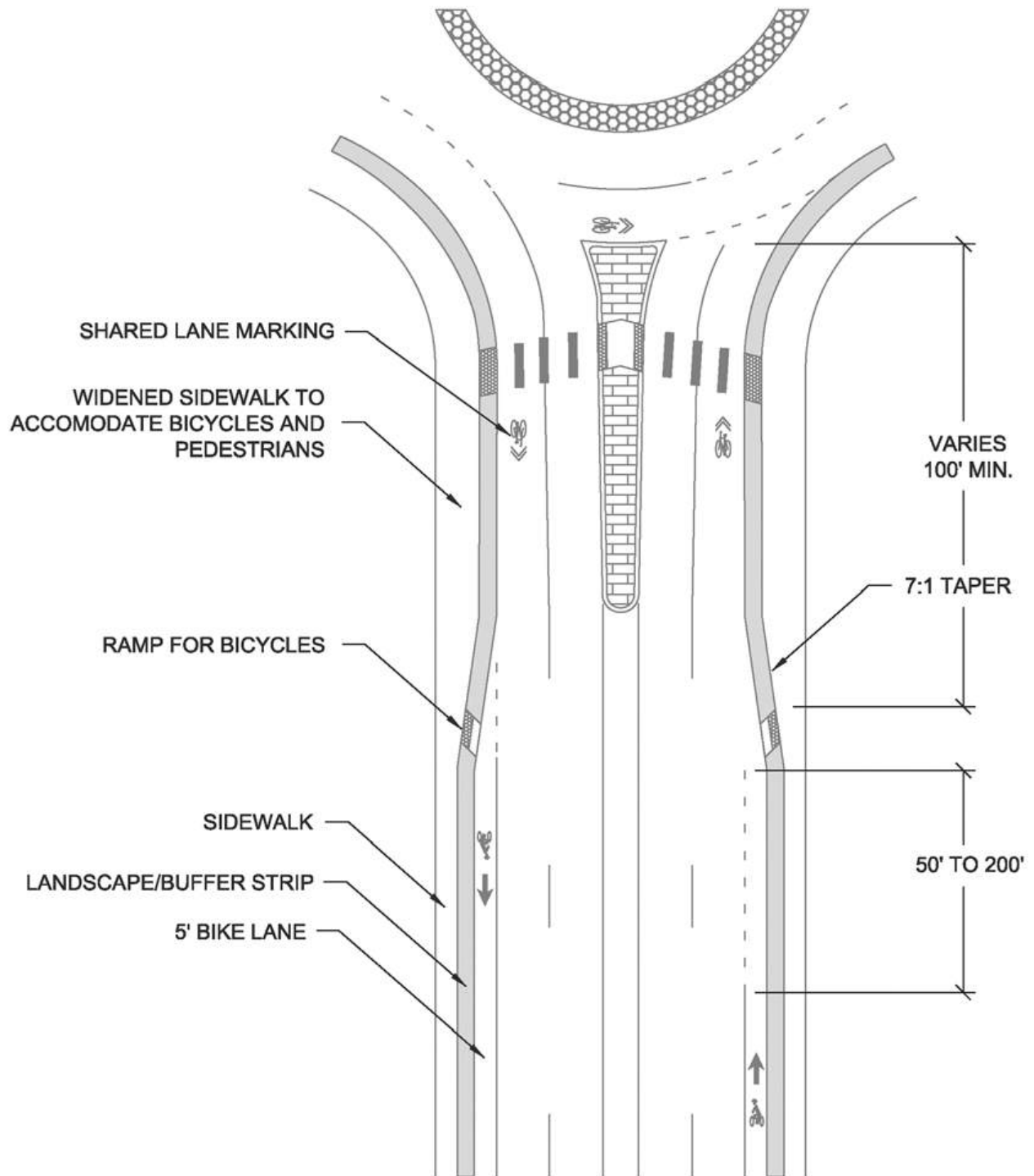
Figure 13-34 Multilane Roundabout
