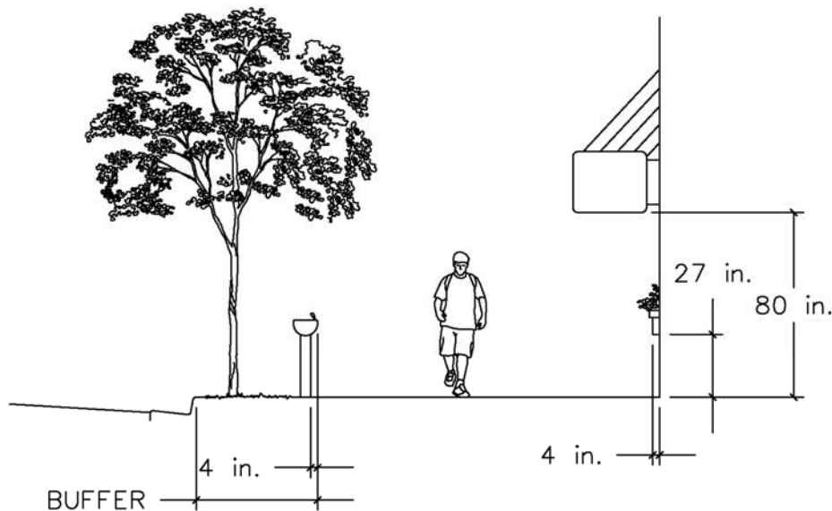
Figure 13-63 Protruding Objects
