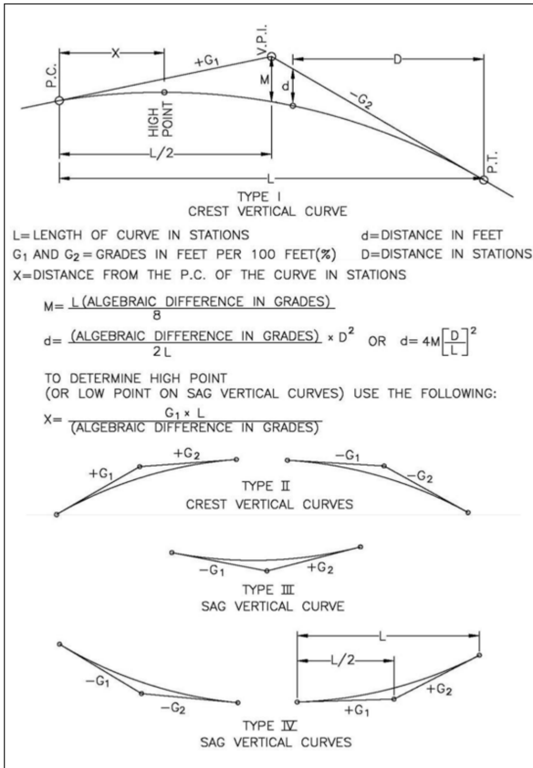
Figure 6-13 Vertical Curves
