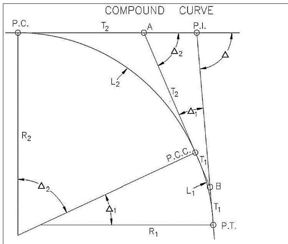
Figure 6-9 Compound Curve
