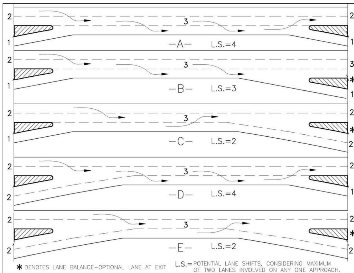
Figure 10-2C Lane Configuration of Weaving Sections
