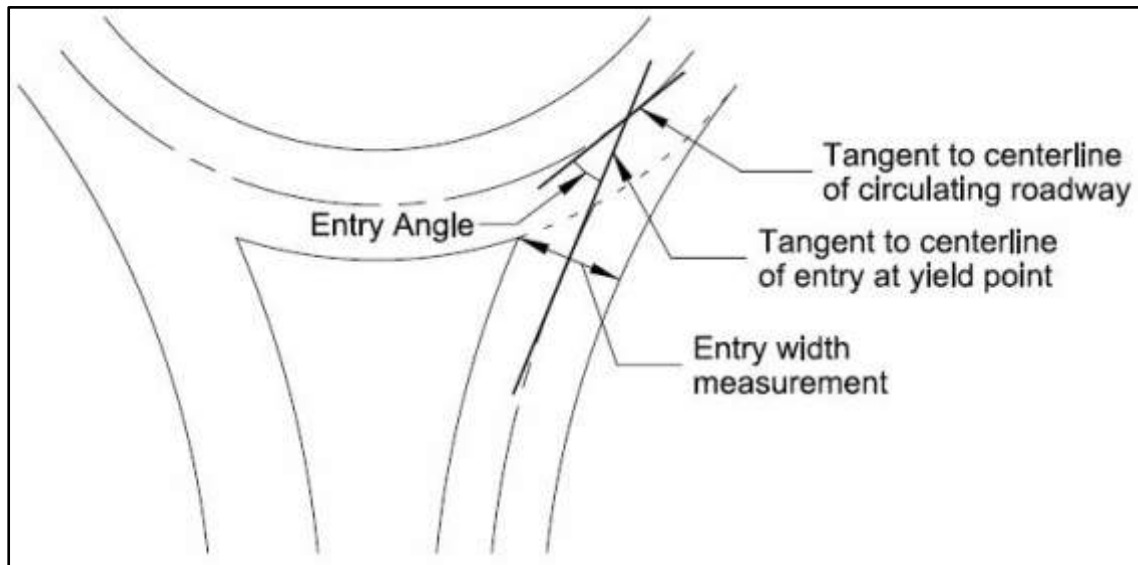
Figure 9-11 Roundabout Entry Angle
