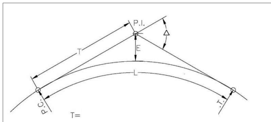
Figure 6-6 Simple Curve
