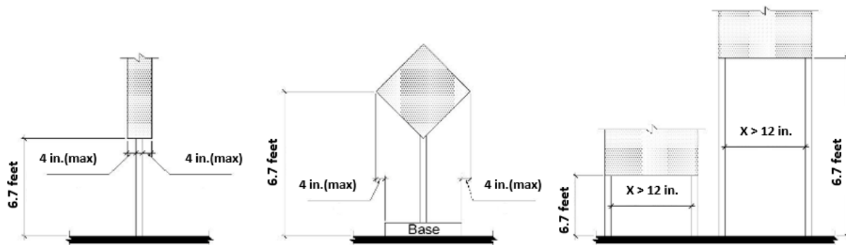
Figure 12-9 Post-Mounted Objects
