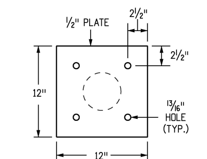
BOTTOM SUPPORT PLATE
