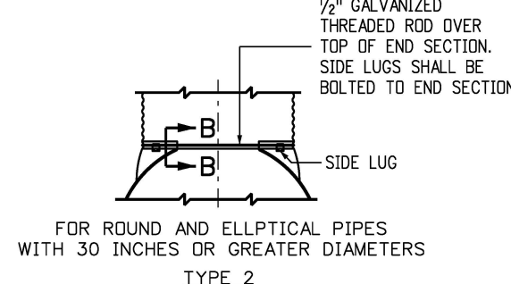
ELEVATION VIEW CROSS DRAINAGE END SECTION
