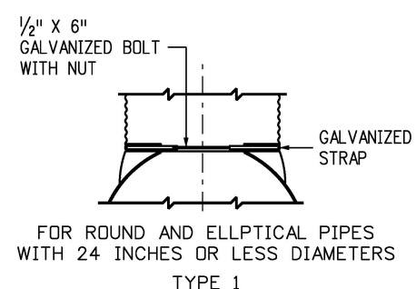
FRONT VIEW ROUND PIPE CULVERT
