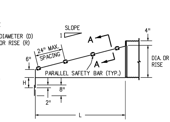
ELEVATION VIEW PARALLEL DRAINAGE END SECTION
