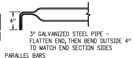
SAFETY BAR DETAILS
