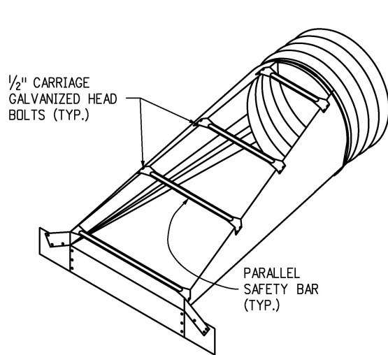
PARALLEL DRAINAGE END SECTION
