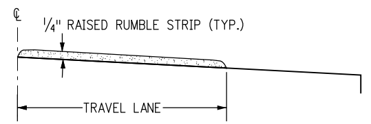
SECTION B-B (RAISED) TEMPORARY RAISED RUMBLE STRIPS
