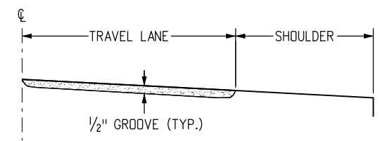
SECTION B-B (GROOVED) PERMANENT GROOVED RUMBLE STRIPS
