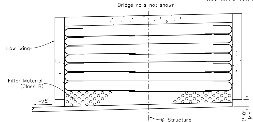
SECTION A
