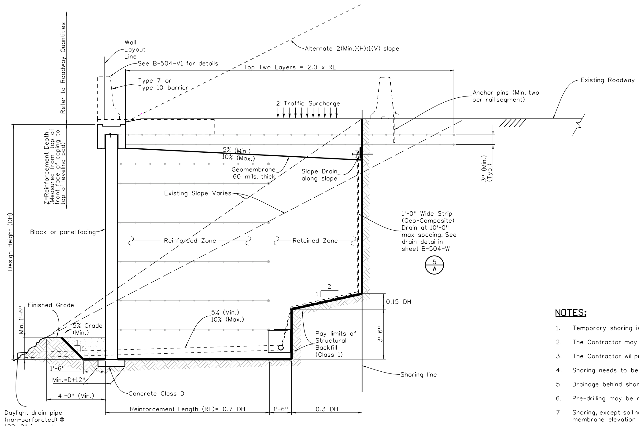
SECTION VIEW
