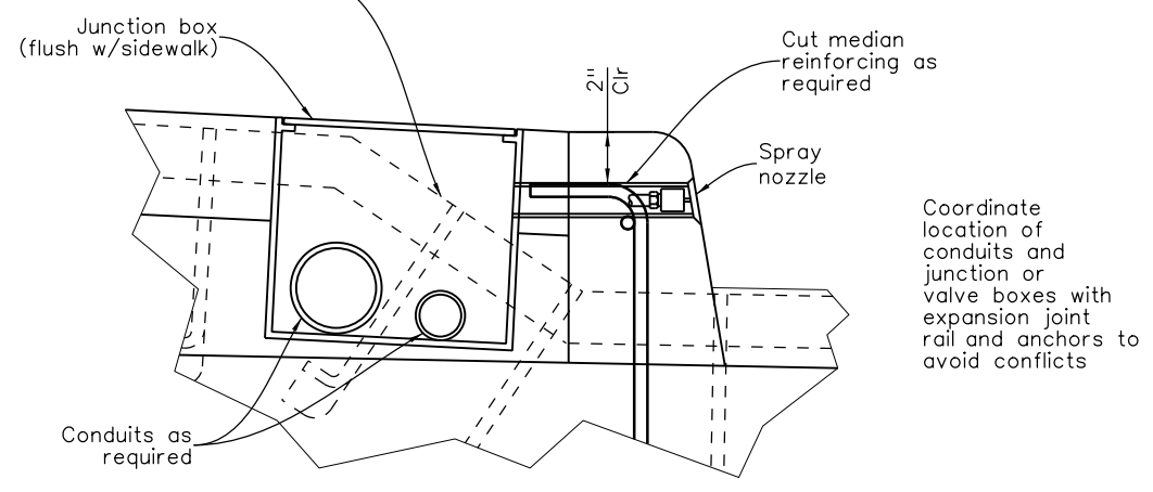
MEDIAN VALVE JUNCTION BOX ON BRIDGE
