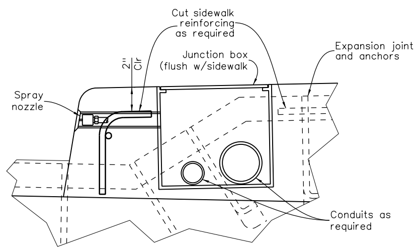
SIDEWALK VALVE JUNCTION BOX ON BRIDGE
