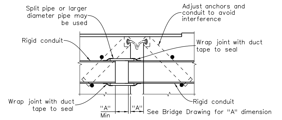
UTILITY CONDUIT DETAIL AT EXPANSION JOINT ON BRIDGE
