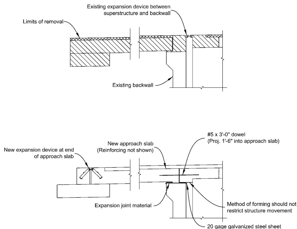
Figure 33-3: Expansion Joint Relocation
