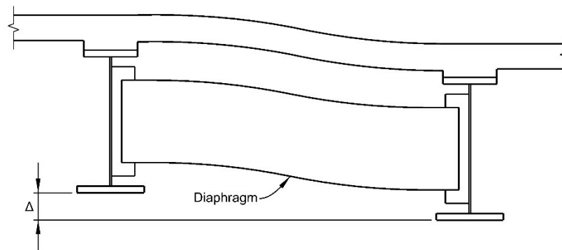
Figure 33-4: Differential Deflection
