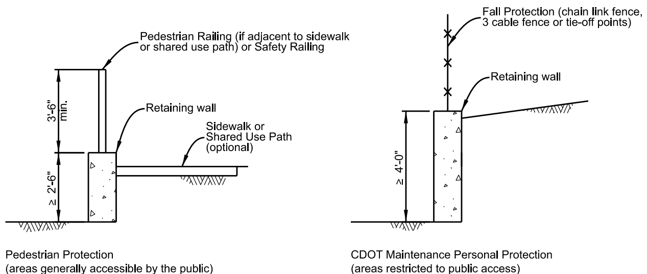
Figure 2-8: Drop-Off Protection
