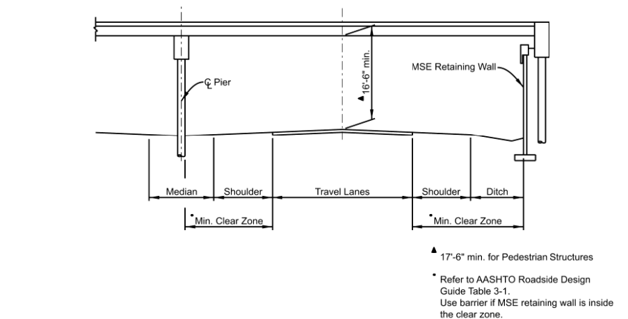
Figure 2-3: Bridge Clearances with MSE Retaining Wall
