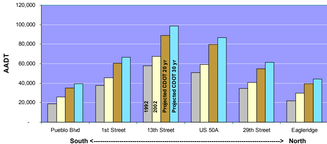
Figure 6-10: I-25 Daily Traffic, 1992 - 2030
