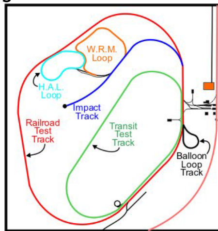
Figure 2.14 TTCI Rail Facilities
