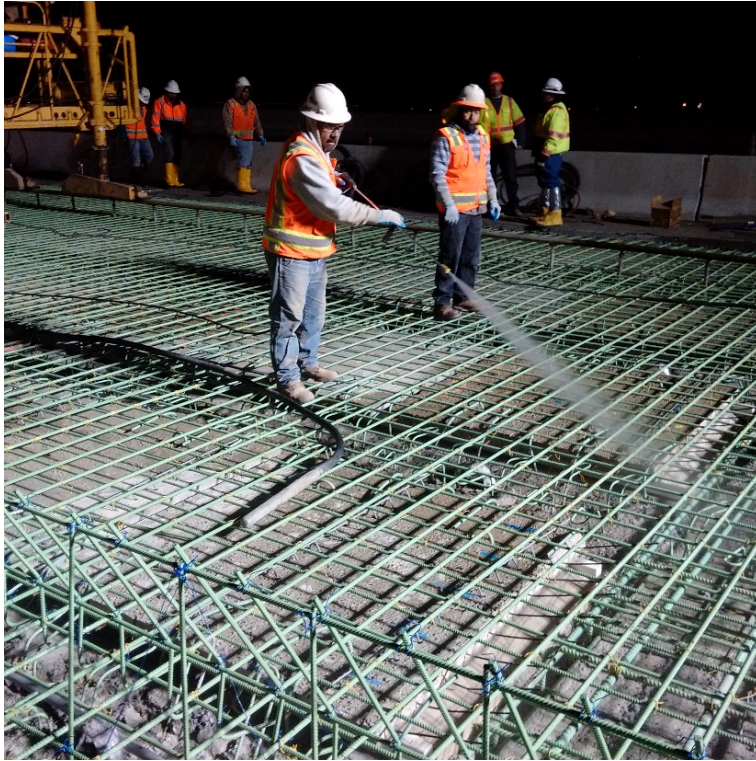
Figure 4-2. Rebar installation
