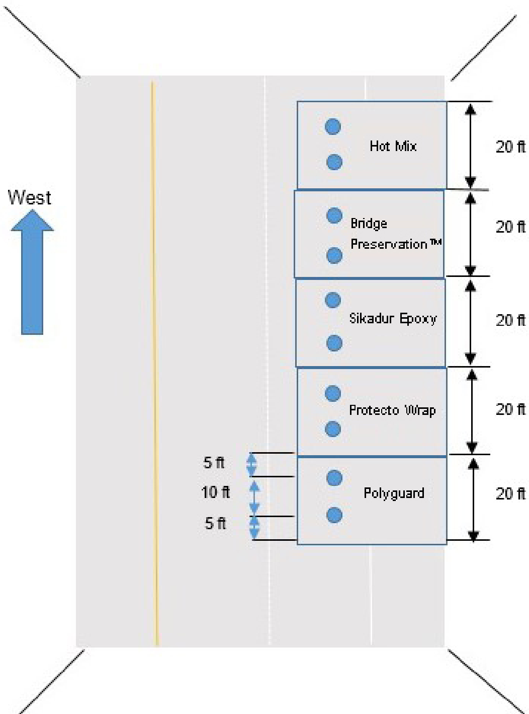
Figure 4-1. Plan view of test sections
