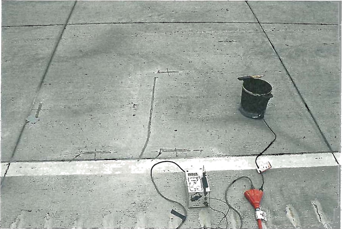
Figure C.5 - Typical Strain Gage Layout at CDOT Project #3
