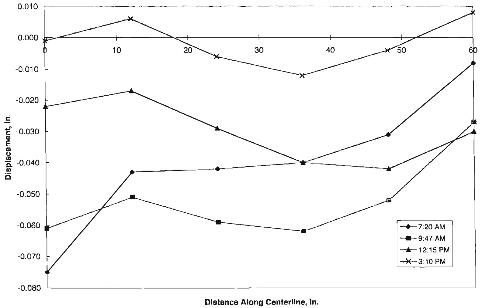
Figure C.8 - Typical Surface Profiles Along Section E Slab Centerline, CDOT Project #3
