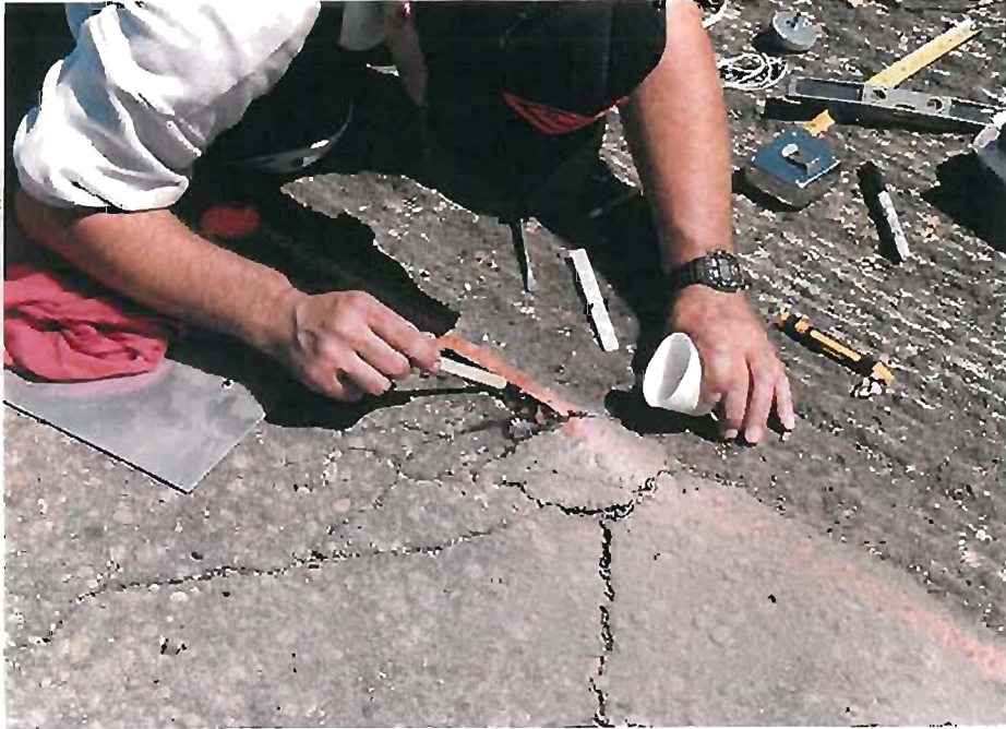
Figure B.7 - Installing Strain Gages on the Asphalt Concrete Surface at CDOT Project #2
