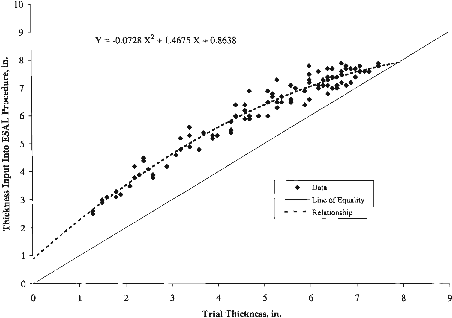
Figure 6.2.1 - Thickness Conversion from Mechanistic Procedure to Empirical Procedure
