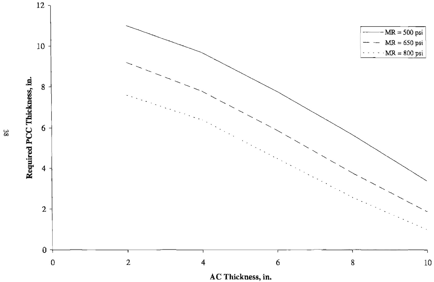
Figure 7.0.4 - PCC Thickness Sensitivity to Concrete Flexural Strength
