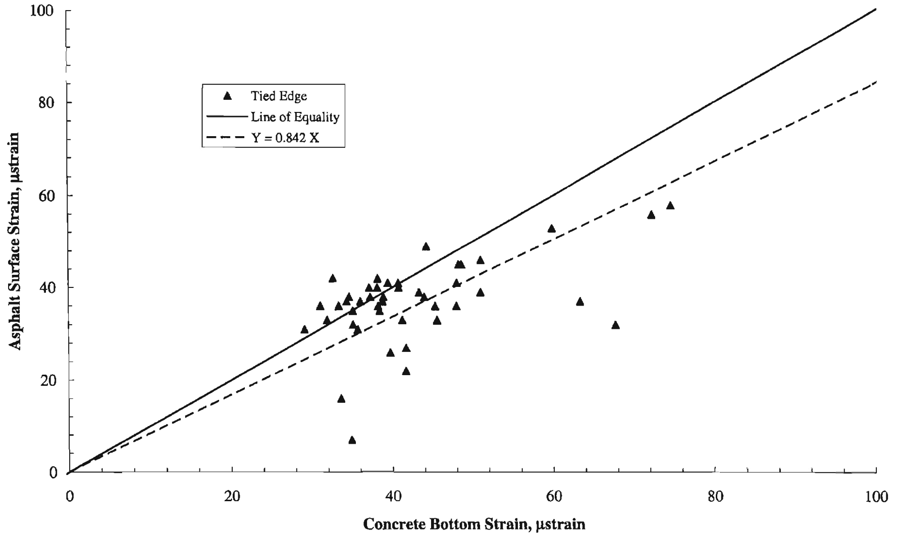
Figure 5.4.1 - Asphalt Surface Strain vs. Concrete Bottom Strain
