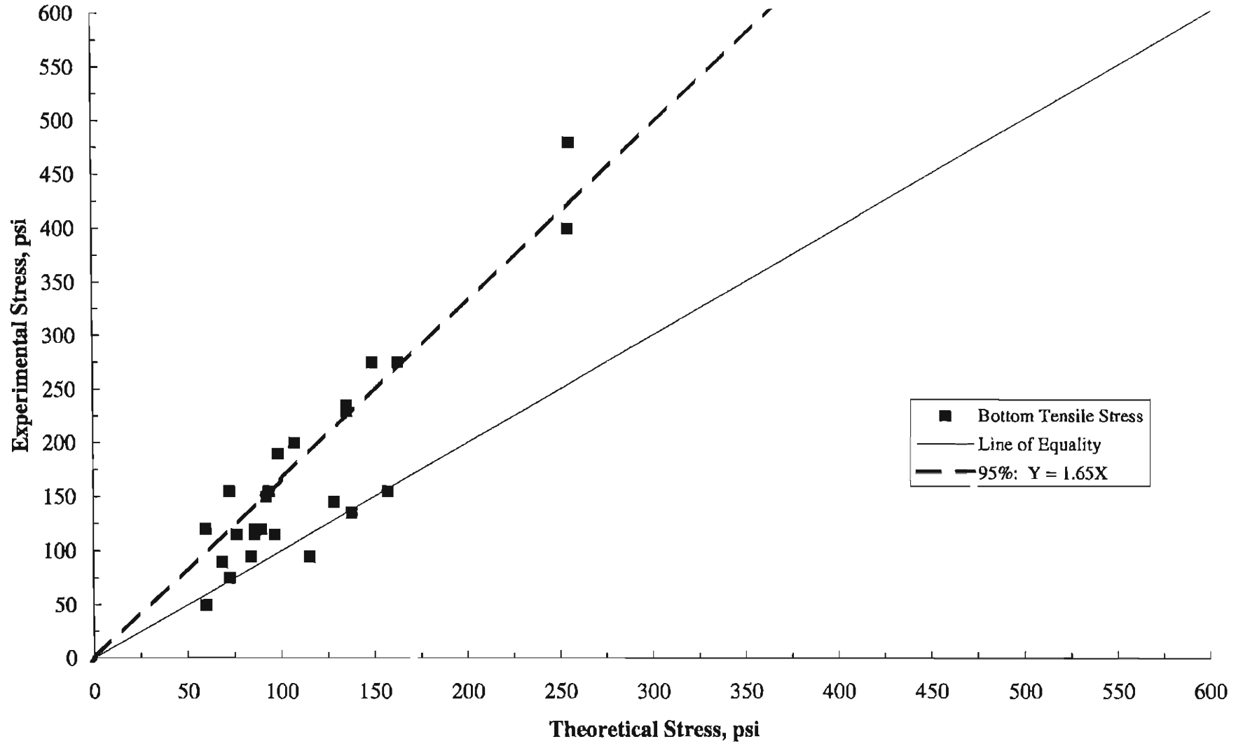
Figure 5.3.1 - Increase in Critical Load Stress Due to Partial Bonding Condition
