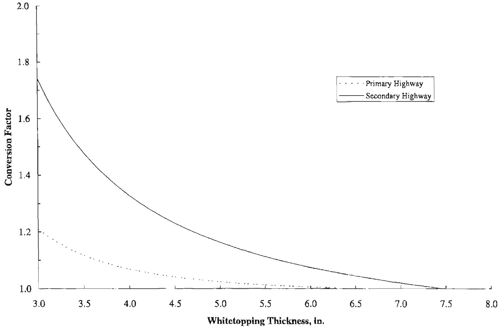
Figure 6.1.1 - Conversion of 8-in.-thick ESALs to Whitetopping ESALs
