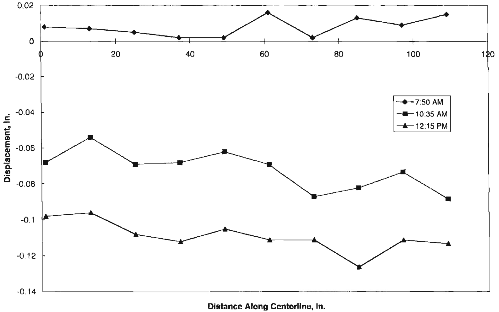
Figure B.14 - Typical Surface Profiles Along Centerline of Slab 2, CDOT Project #2 28-Day Testing
