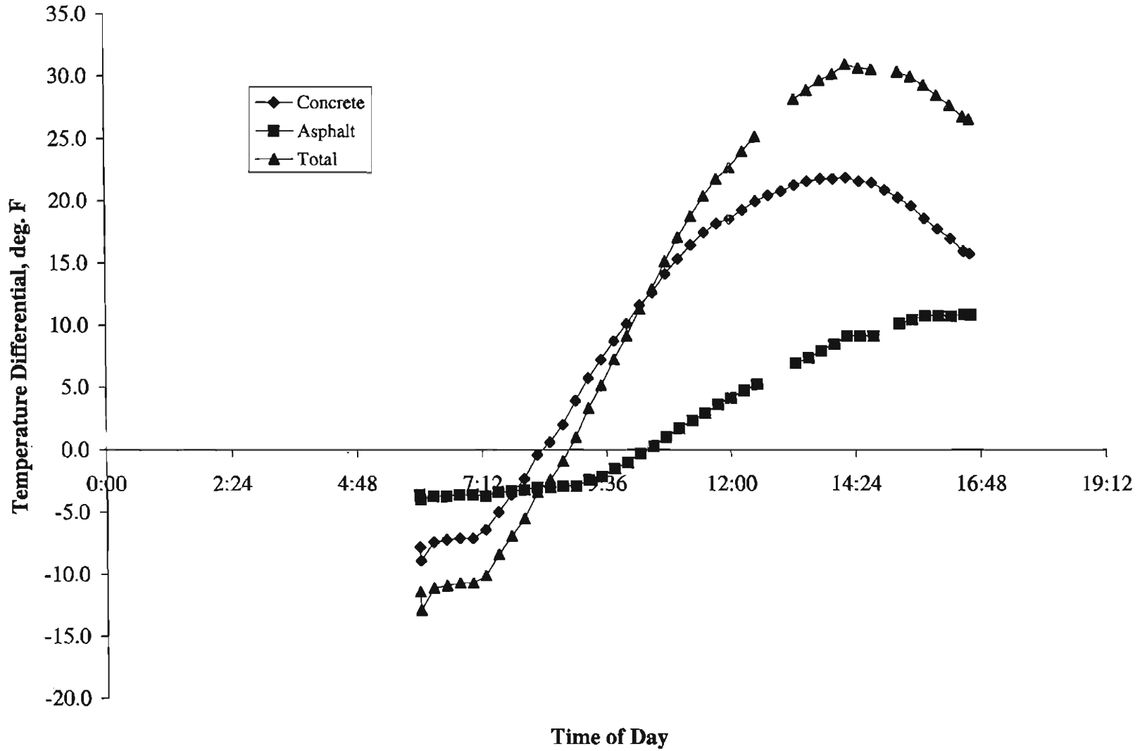
Figure A.10 - Typical Temperature Gradient in CDOT1 Pavement Layers
