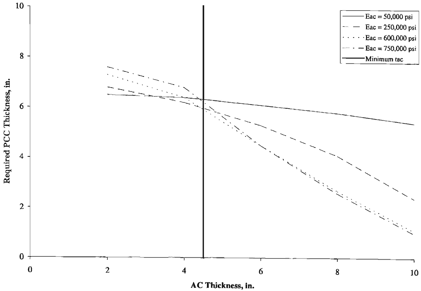
Figure 7.0.3 PCC Thickness Sensitivity to AC Modulus of Elasticity
