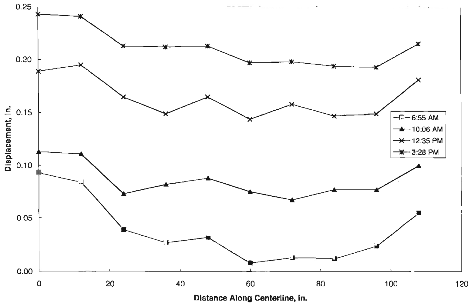
Figure C.7 - Typical Surface Profiles Along Section B Slab Centerline, CDOT Project #3
