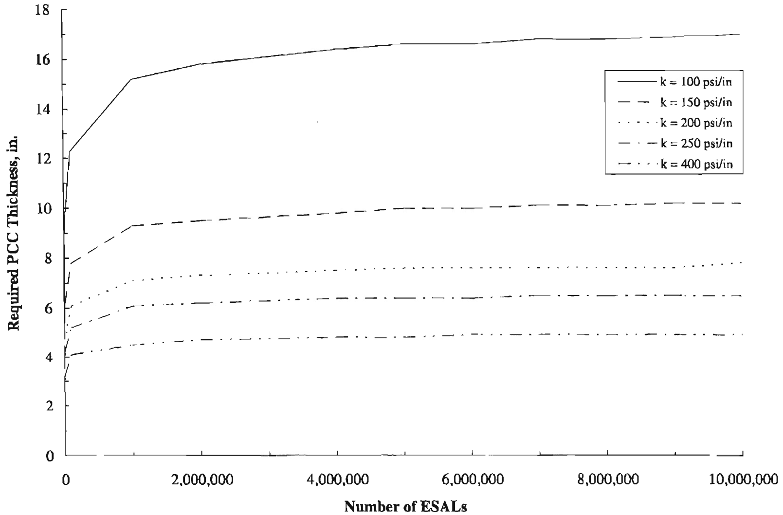
Figure 7.0.8 - PCC Thickness Sensitivity to Modulus of Subbase/Subgrade Reaction
