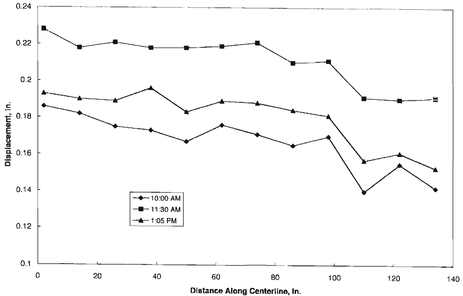
Figure B.16 - Typical Surface Profiles Along Centerline of Slab 5, CDOT Project #2 28-Day Testing
