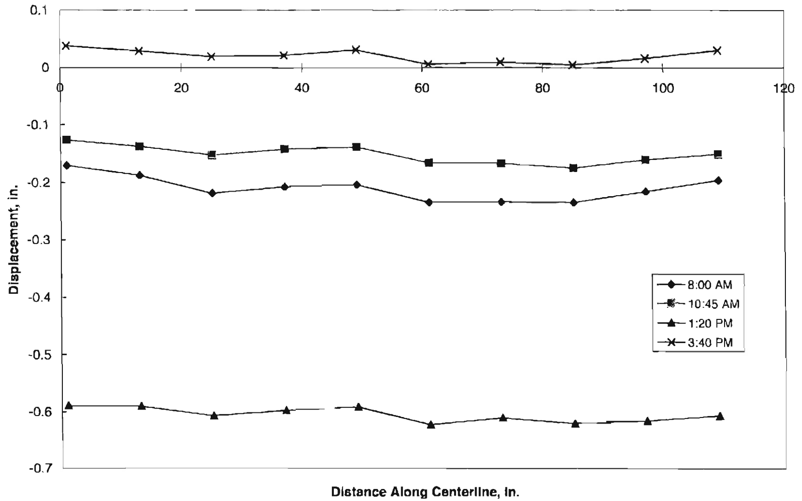
Figure B.15 - Typical Surface Profiles Along Centerline of Slab 2, CDOT Project #2 365-Day Testing
