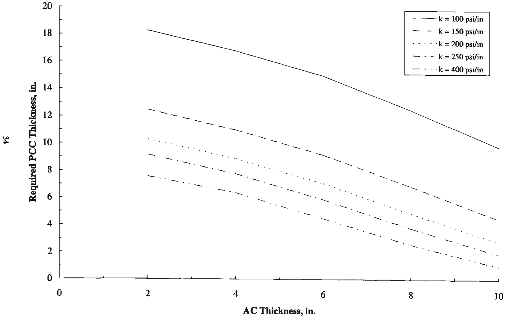
Figure 7.0.1 - PCC Thickness Sensitivity to Modulus of Subbase/Subgrade Reaction
