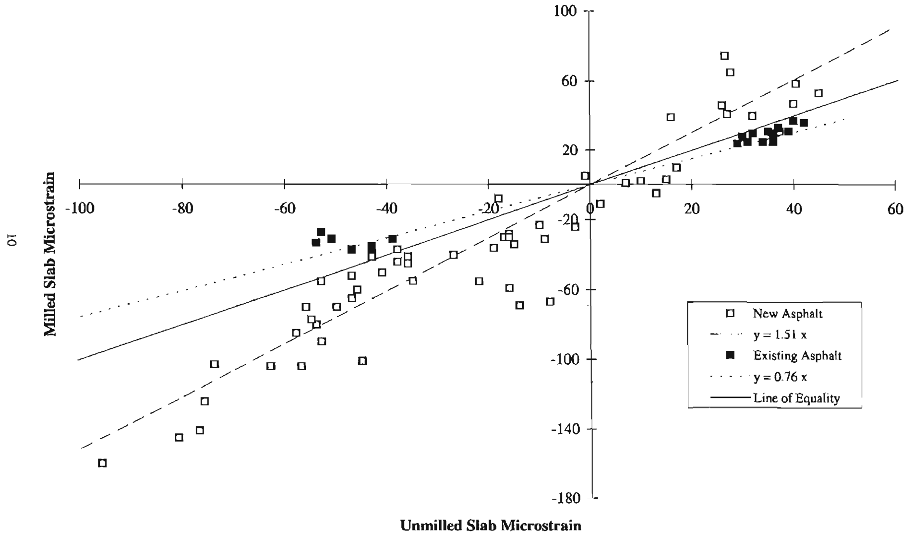
Figure 4.5.1- Effect of Interface Milling on Load Induced Microstrain
