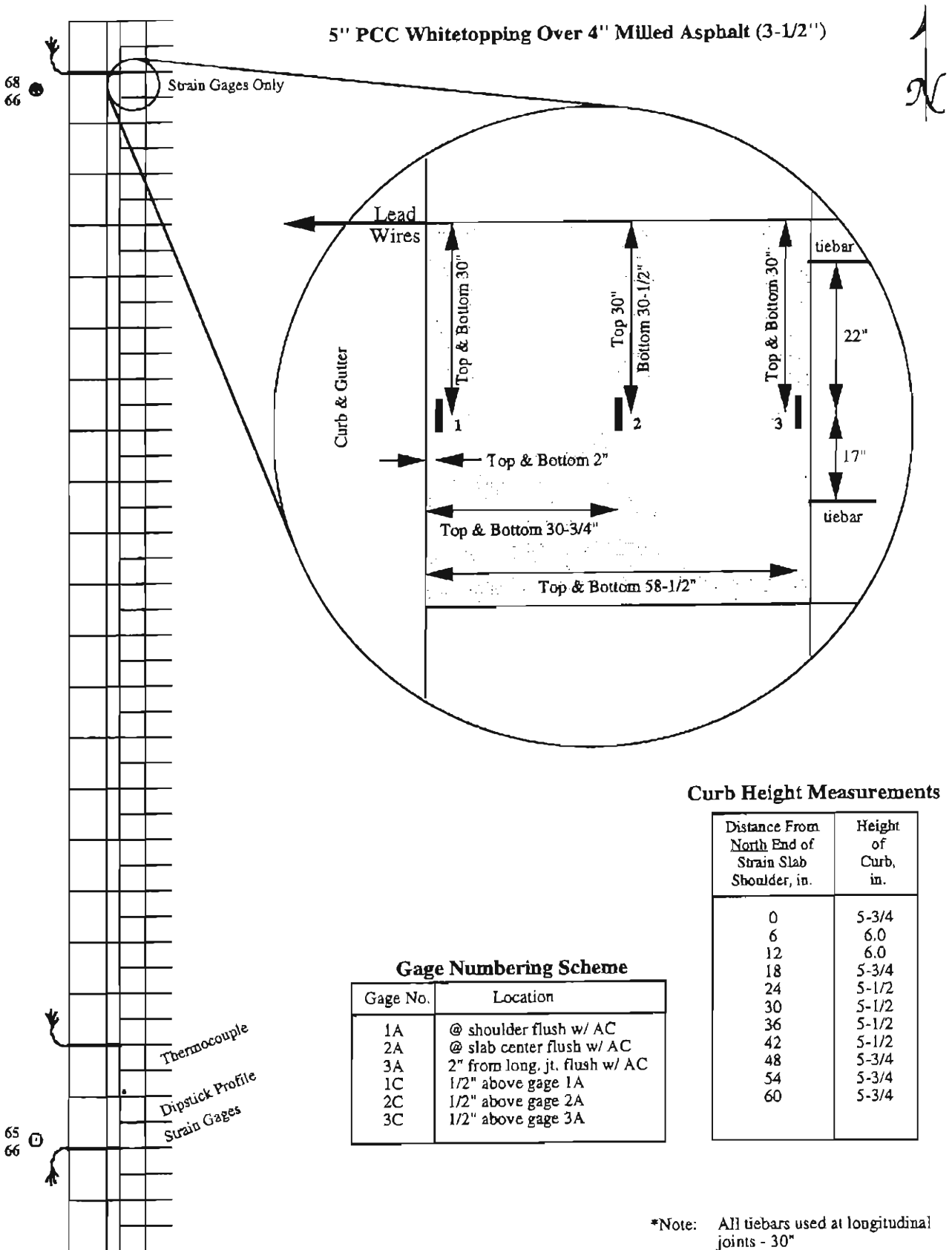
Figure A.3 - Test Slab 3 Layout for CDOT Project #1.
