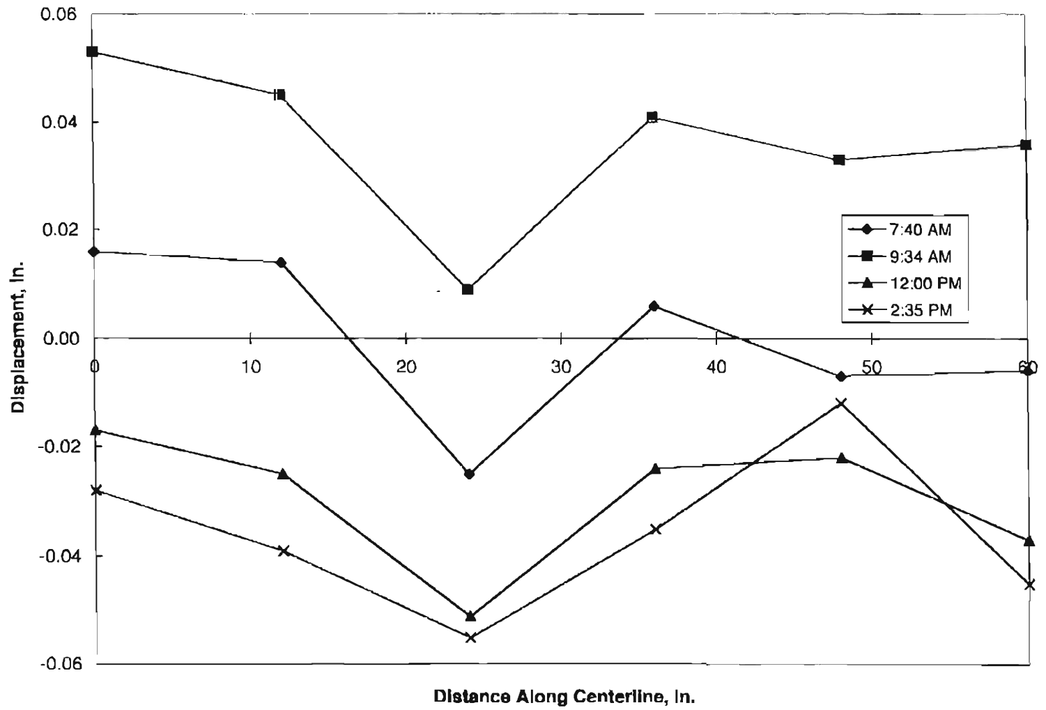
Figure C.9 - Typical Surface Profiles Along Section F Slab Centerline, CDOT Project #3
