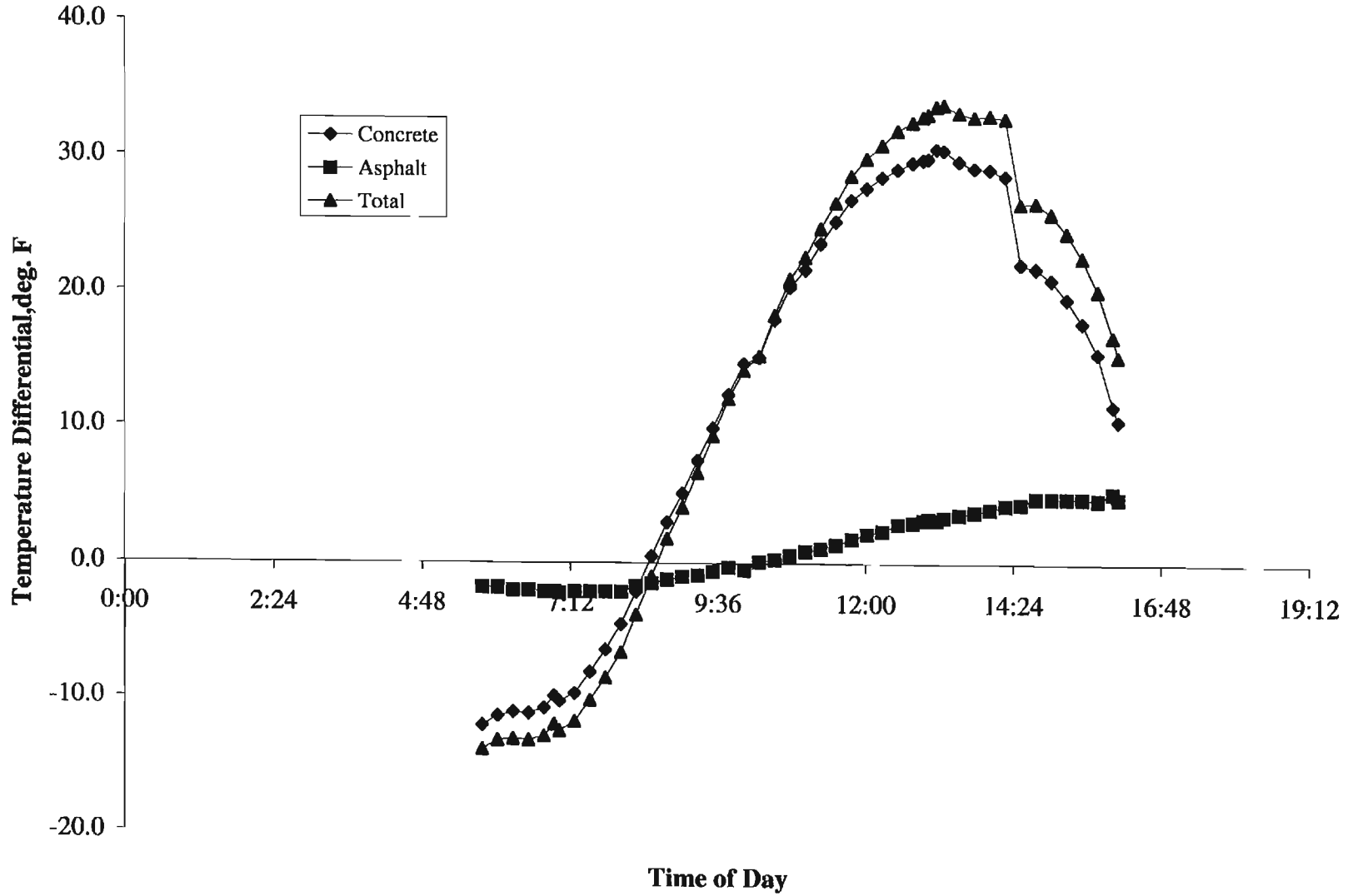
Figure B.6 - Typical Temperature Gradient in CDOT2 Pavement Layers
