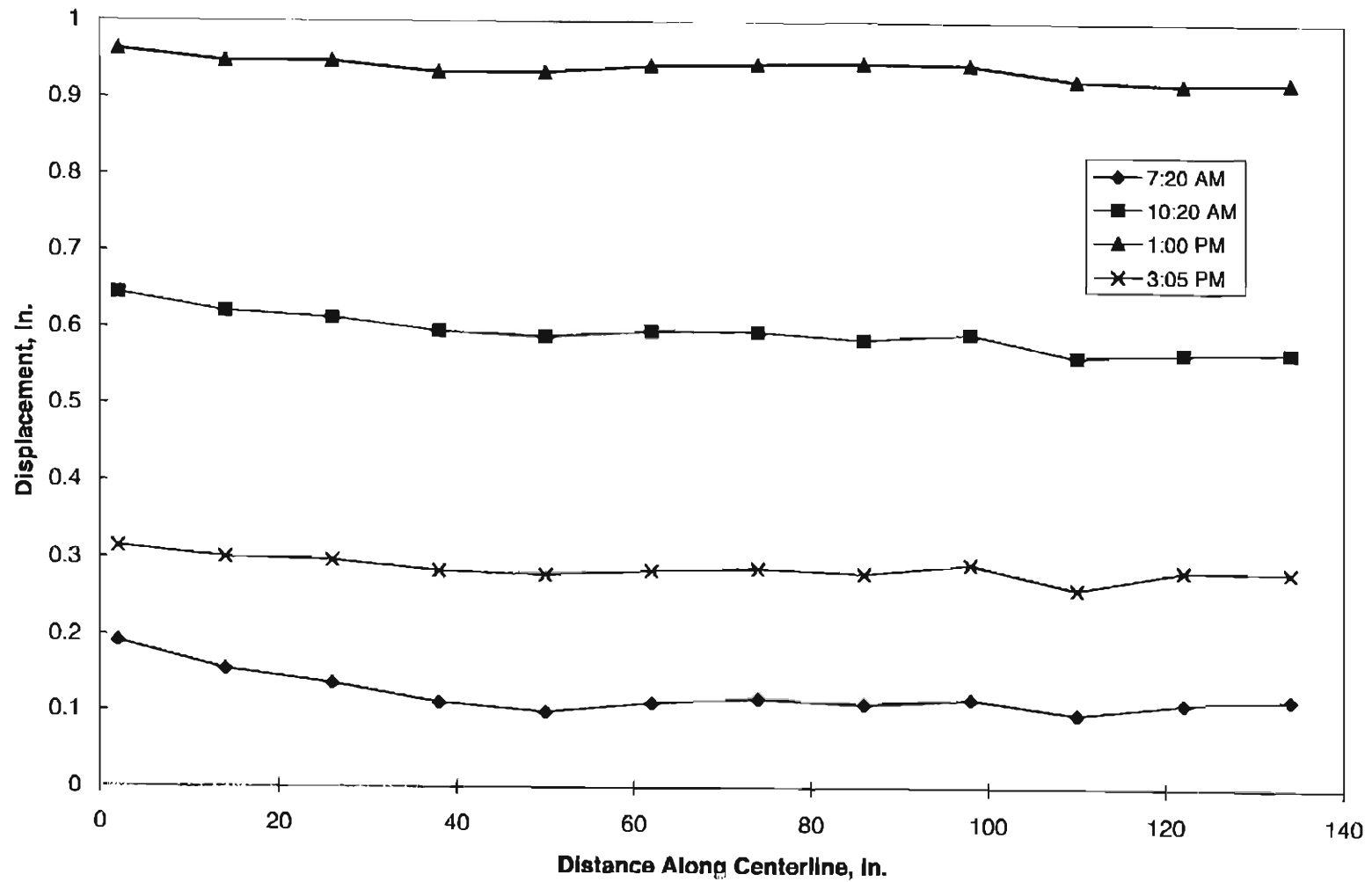
Figure B.17 - Typical Surface Profiles Along Centerline of Slab 5, CDOT Project #2 365-Day Testing
