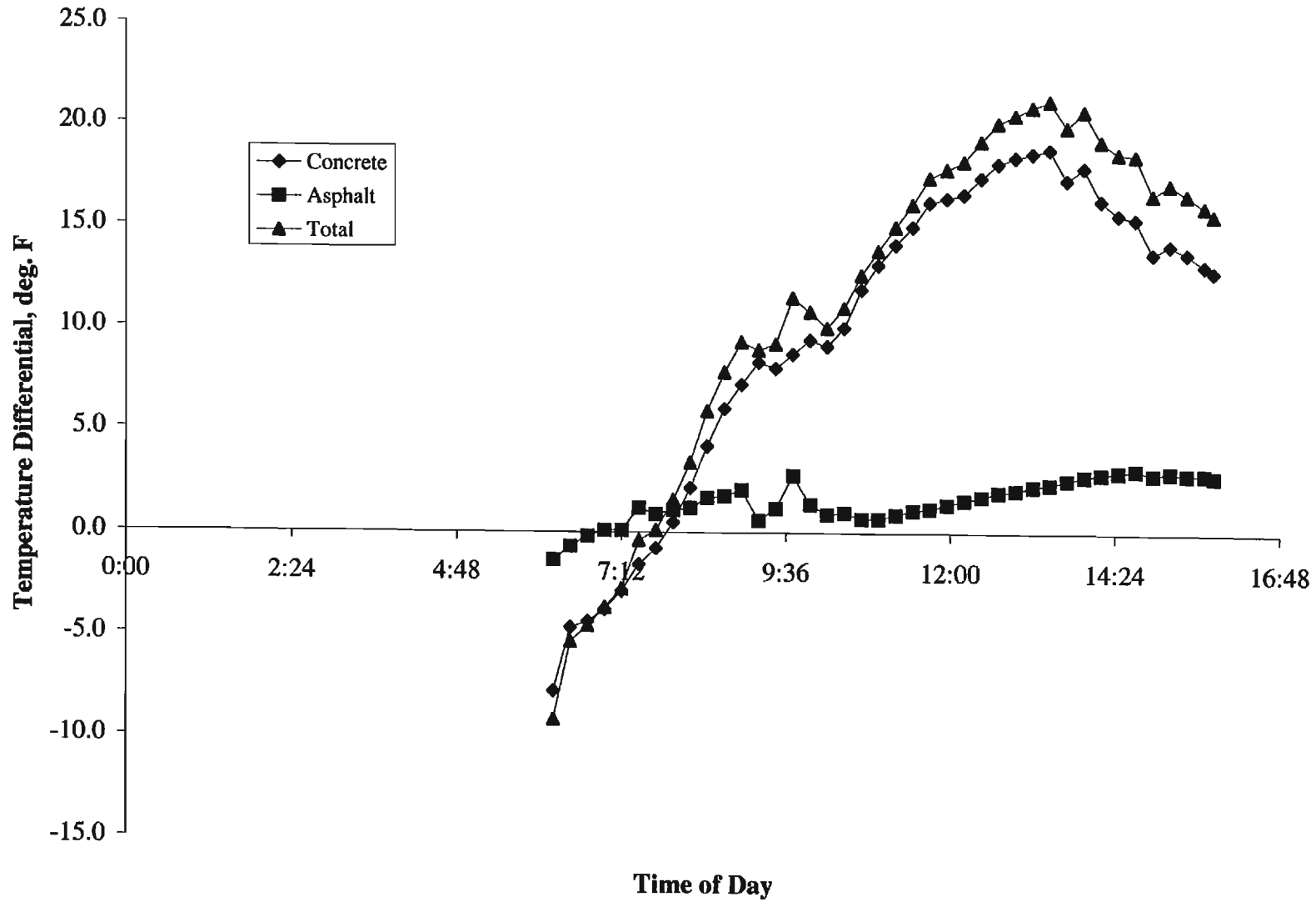
Figure C.4 - Typical Temperature Gradient in CDOT3 Pavement Layers
