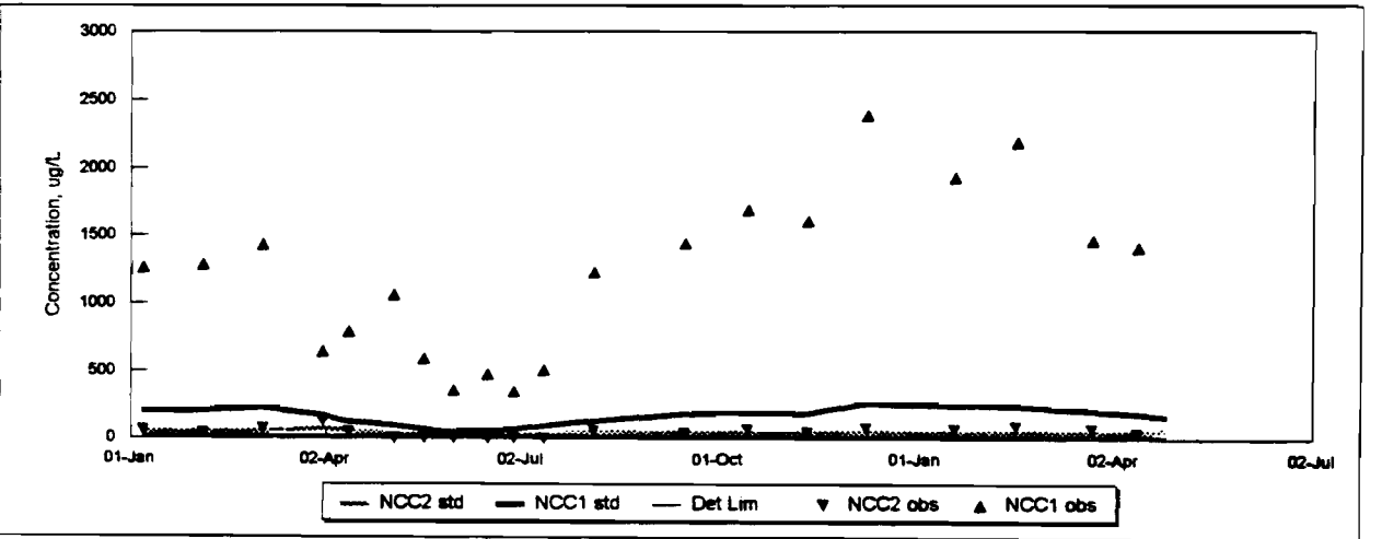
Figure 20. Total recoverable zinc (points) and standards for zinc (lines: soluble, chronic).
