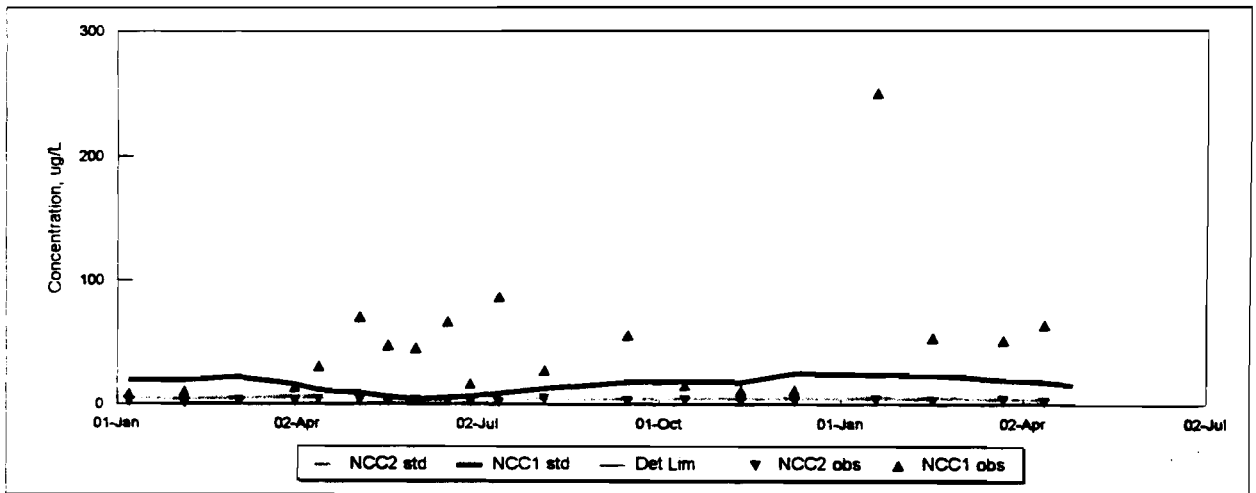
Figure 19. Total recoverable copper (points) and standards for copper (lines: soluble, chronic).
