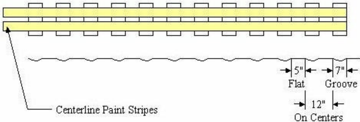
Figure 3. A drawing of the centerline rumble strips.
