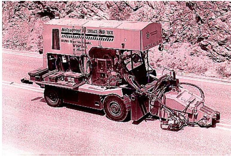
Figure 2. The machine that grinds the rumble strips
