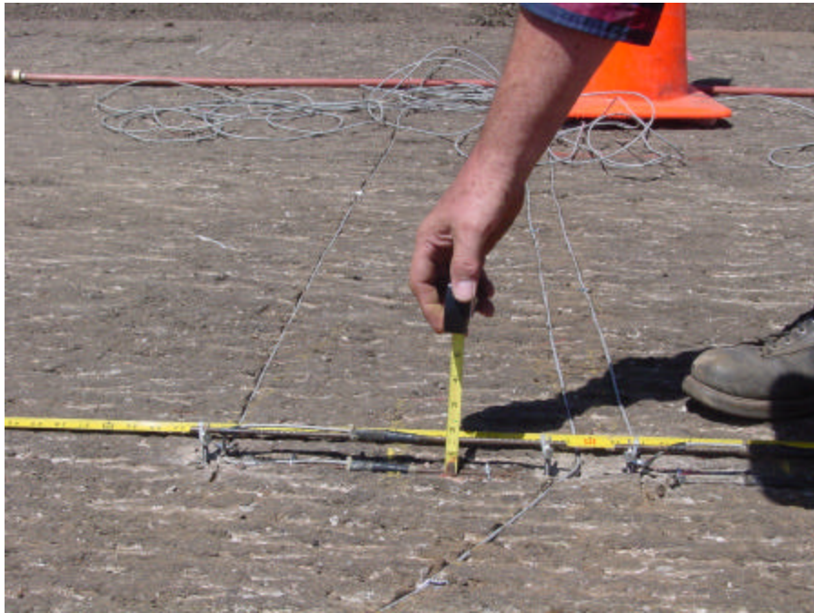
Figure 14. Embedded Strain Gages
