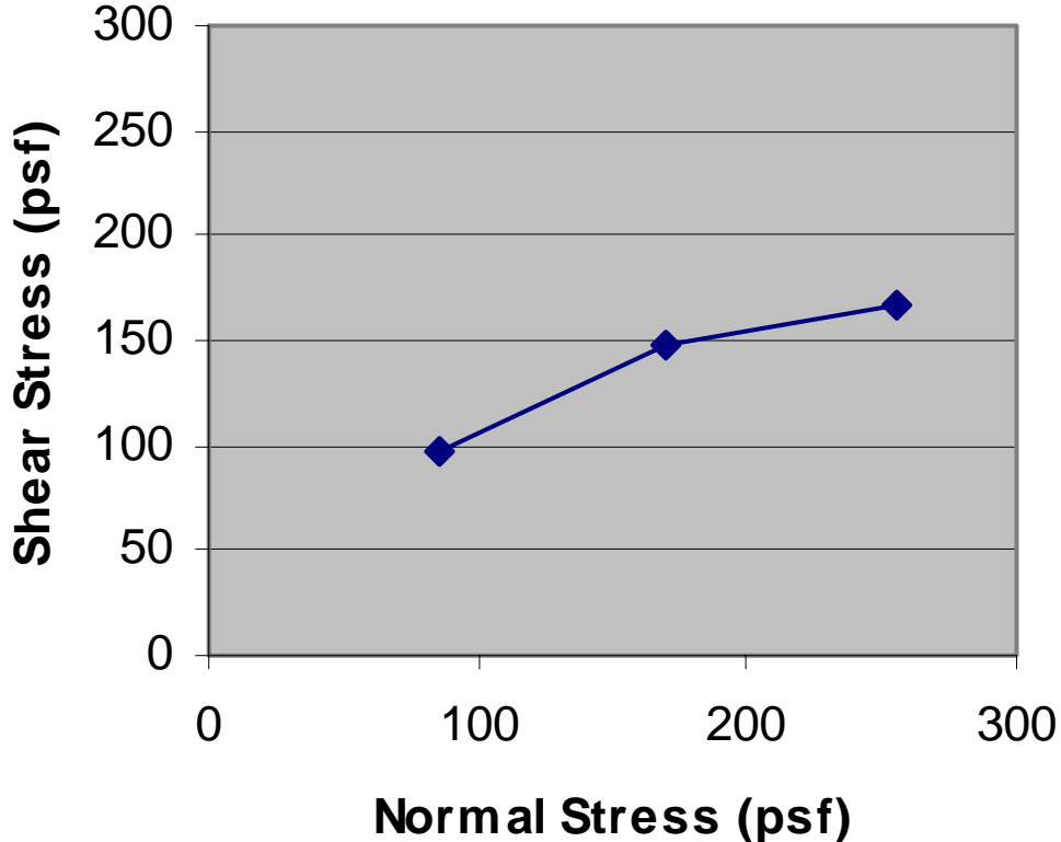
Figure 4.7. Shear at interface between two vertically stacked tire bales (1 psf = 48 Pa)
