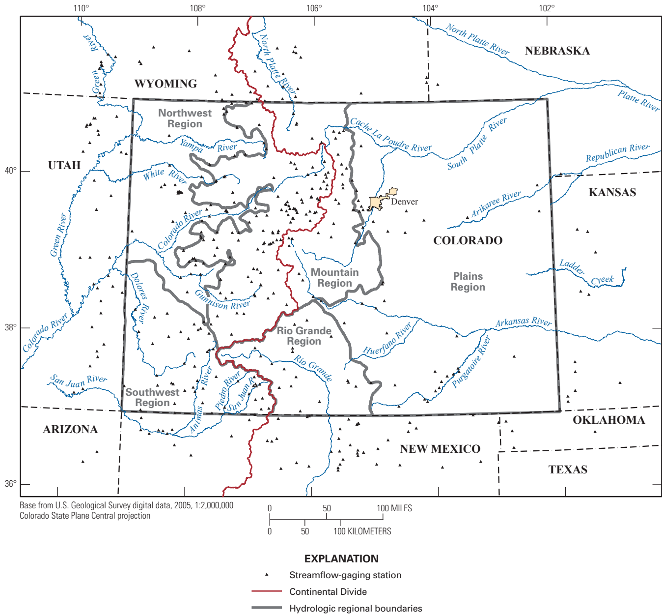
Figure 1. Boundaries of hydrologic regions and locations of streamflow gaging stations in Colorado and adjacent States.
