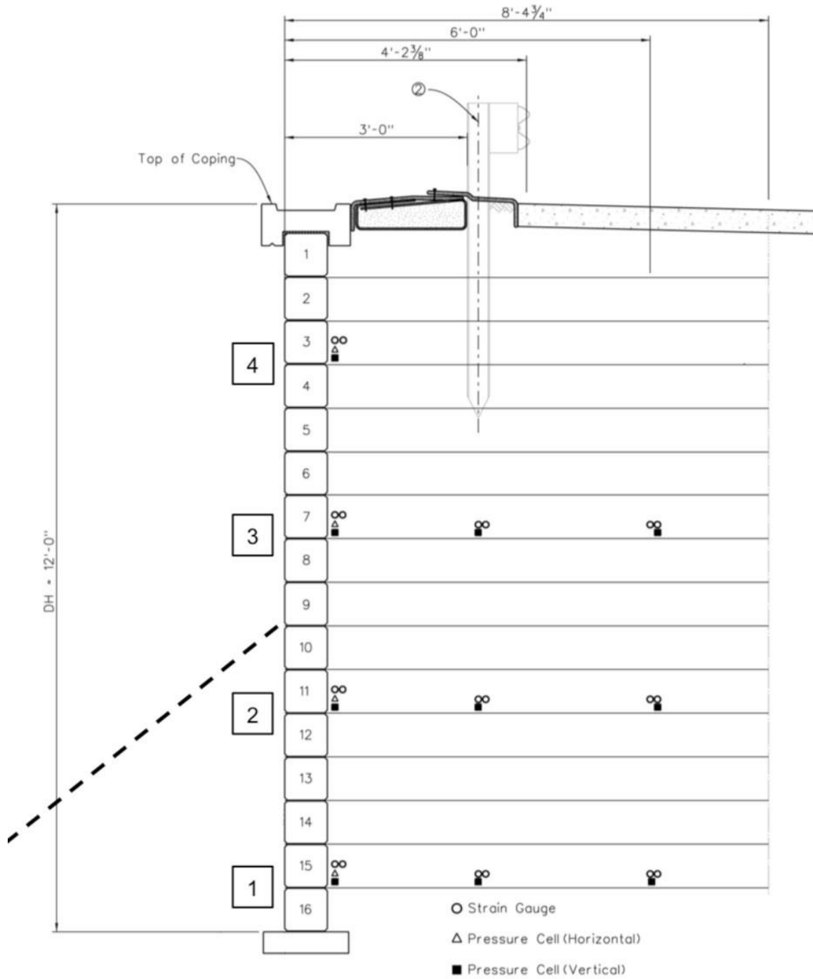
Figure 29. GRS Wall with cells measuring horizontal pressure ( \Delta ) on the facing blocks.
