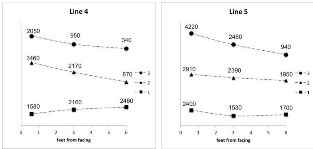
Figure 35. Reinforcement microstrain
