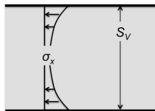
Figure 2. Shear lag in reinforced soil layer
