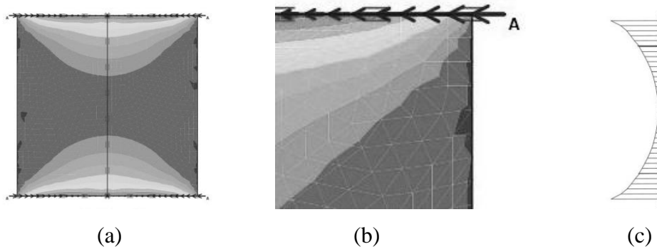
Figure 6. (a) Non-uniform horizontal stress distribution induced by shear, (b) enlargement of corner where shear stress is greatest, and (c) graph of the resulting horizontal stress distribution, which resembles a parabola.
