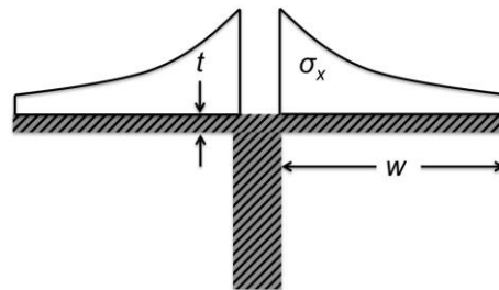
Figure 1. Shear lag in beam flange
