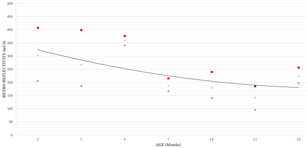
Figure 32. Performance curve obtained in Region 5 when the following criteria was used: LOW, Bituminous Epoxy, Mountainous, and White.
