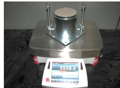
T-99 & T-180 Figure 14: Mass of Mold and Wet Soil
