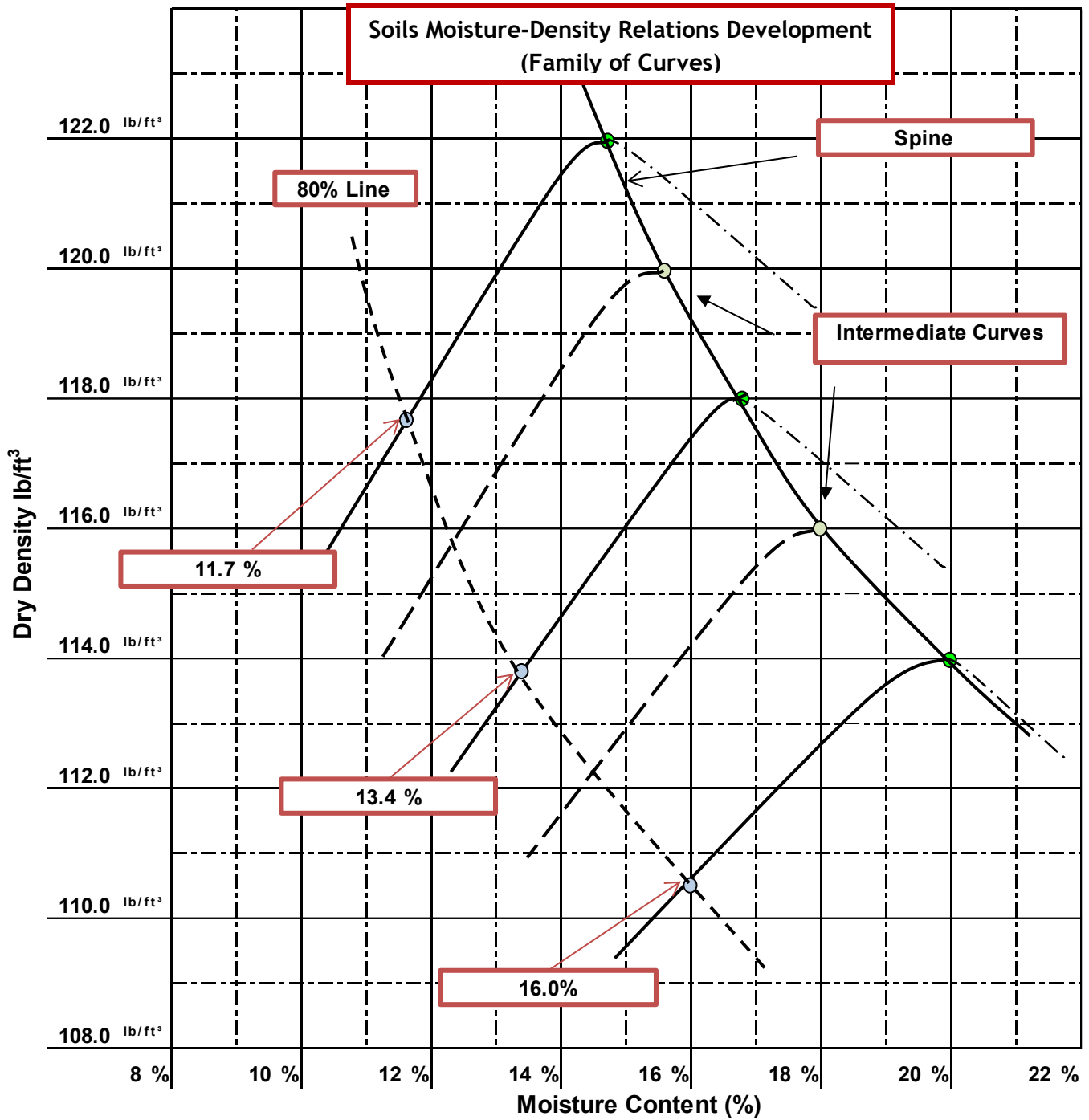
R-75 Figure 2: Example of Moisture-Density Relations Group/Family of Curves
