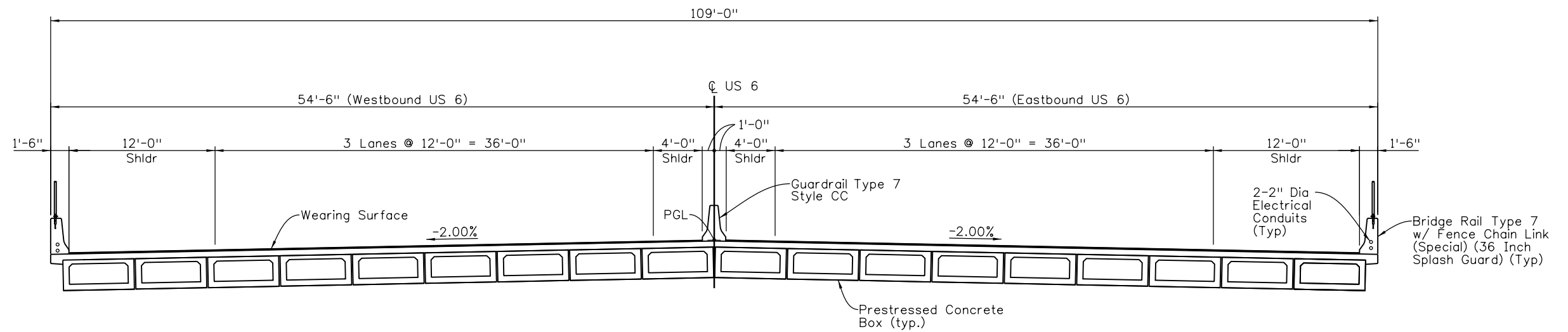
TYPICAL SECTION
