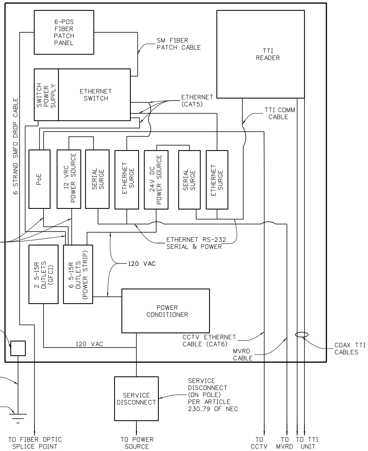
TTI/MVRD/CCTV COMMUNICATIONS CABINET ONE-LINE DIAGRAM FIBER (ETHERNET)
