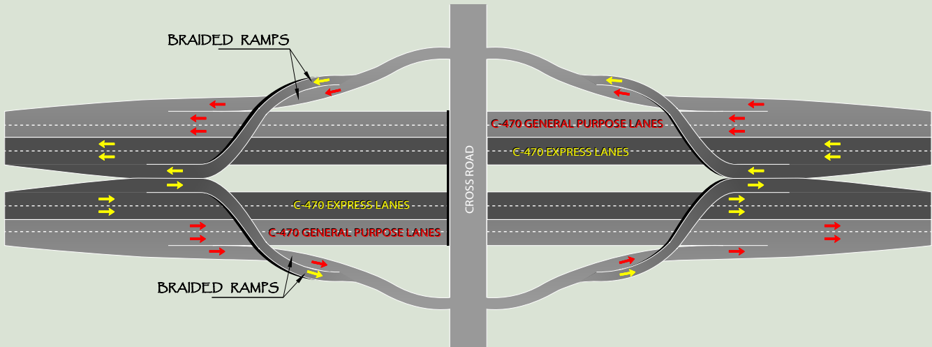
BRAIDED RAMP
