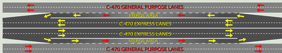
SLIP RAMP
