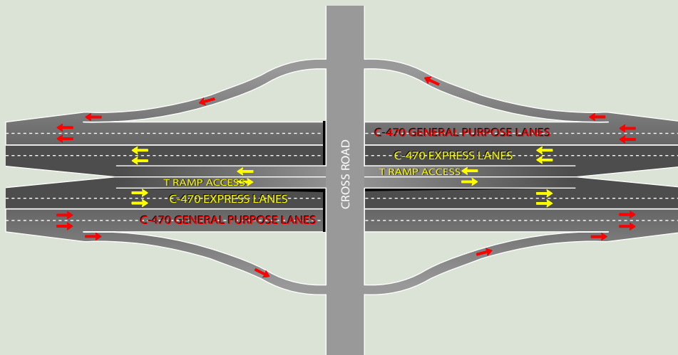
"T"-RAMP
