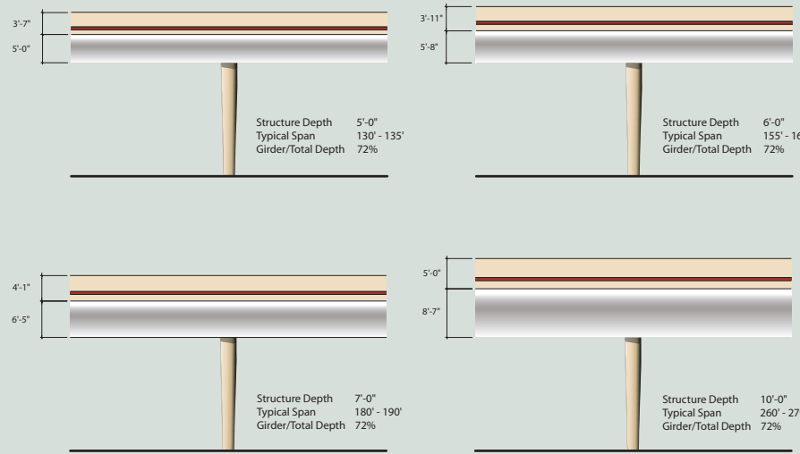
DEPTH RATIOS
