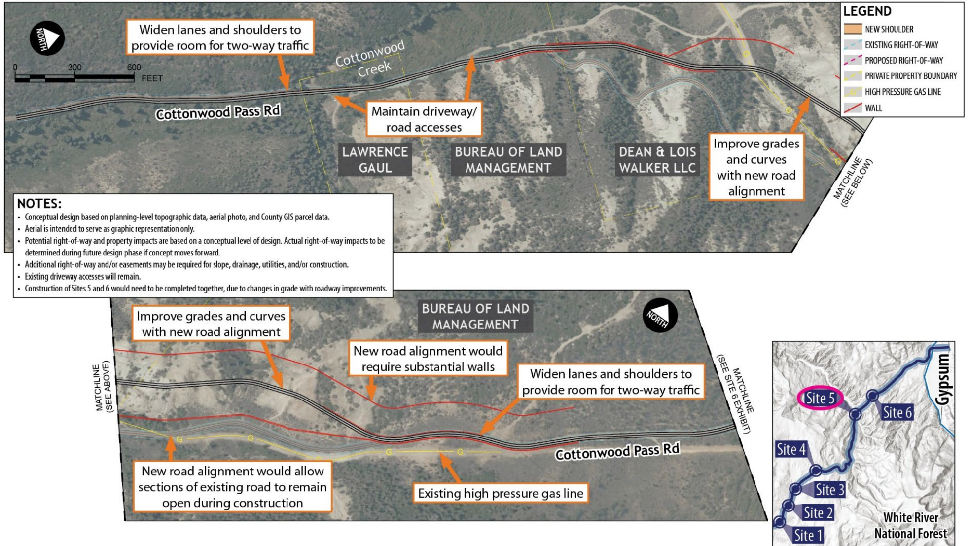
Figure 21. Eagle County Site 5 (Blue Hill) Option 1 - Improved Grades and Curves with New Alignment
