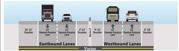
Existing I-270 Cross Section East of Vasquez Boulevard
