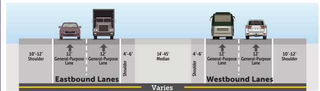
Existing I-270 Cross Section West of Vasquez Boulevard
