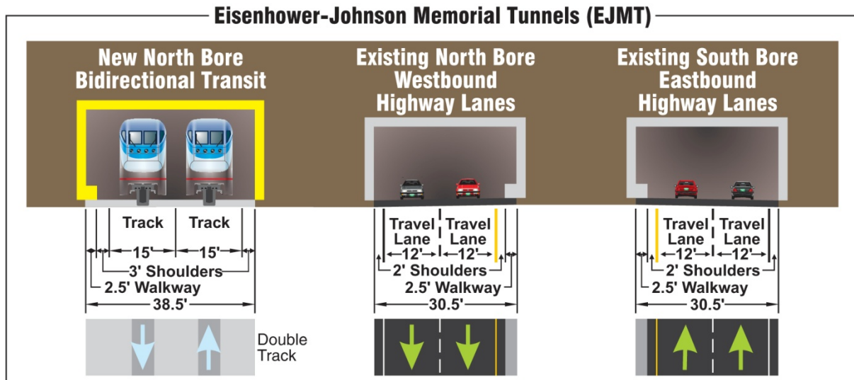
Figure 46. Preferred Alternative (55 and 65 mph Options) Eisenhower-Johnson Memorial Tunnels and Twin Tunnels
