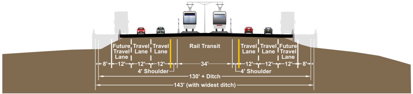
Figure 35. Rail with Highway Preservation
