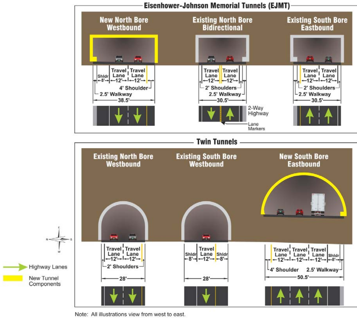
Figure 24. Six-Lane Highway 55 mph Alternative Eisenhower-Johnson Memorial Tunnels and Twin Tunnels
