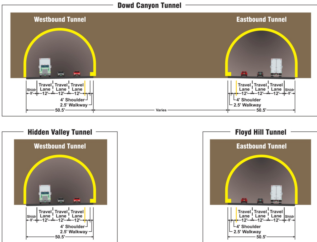
Figure 49. Preferred Alternative (65 mph Option) Dowd Canyon Tunnel, Hidden Valley Tunnel, and Floyd Hill Tunnel
