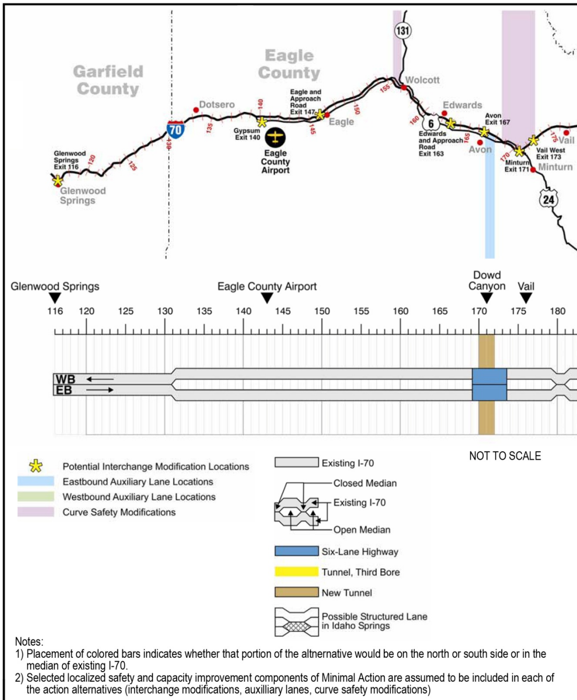
Figure 25. Six-Lane Highway 65 mph Alternative Overview
