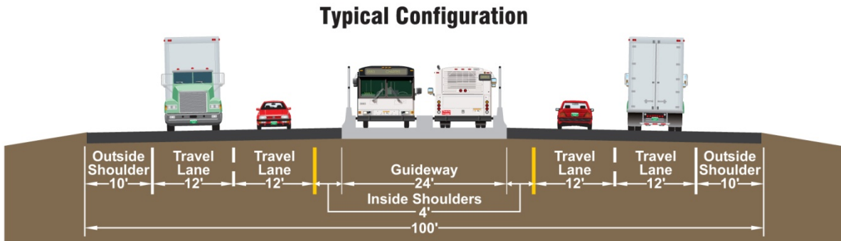
Figure 19. Dual-Mode Bus and Diesel Bus in Guideway Typical Configuration and Elevated Configuration in Idaho Springs
