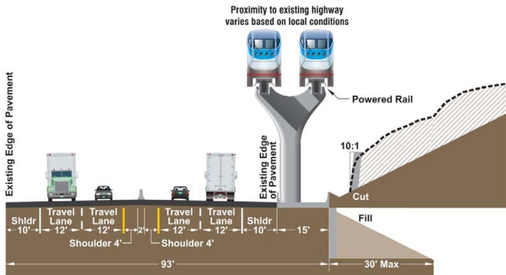
Figure 13. Advanced Guideway System Typical Configuration
