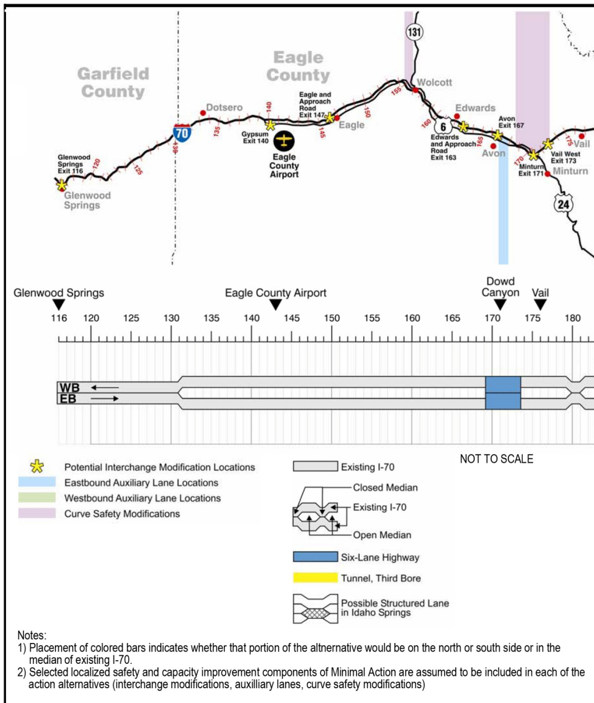
Figure 22. Six-Lane Highway 55 mph Alternative Overview
