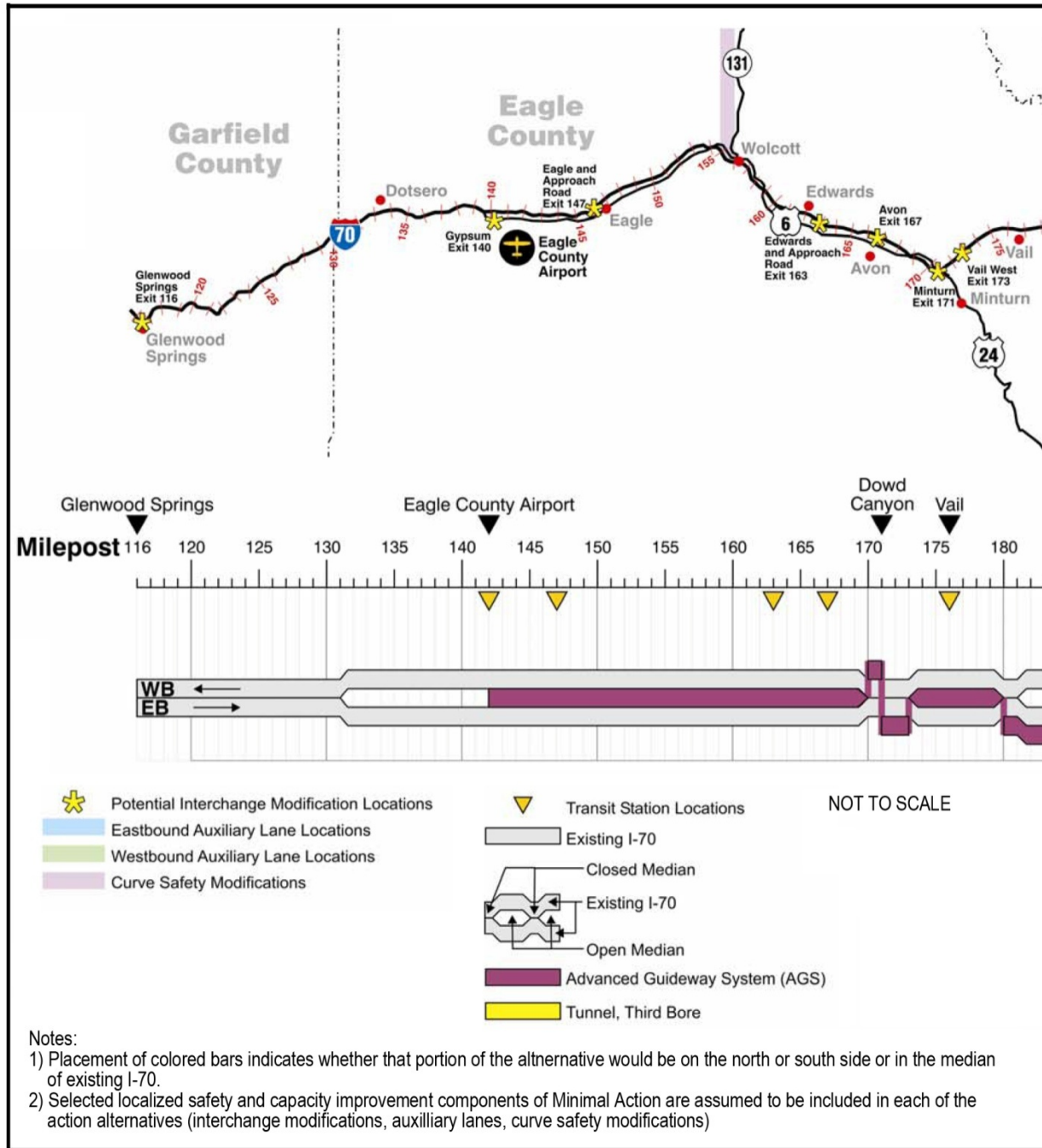
Figure 12. Advanced Guideway System Alternative Overview
