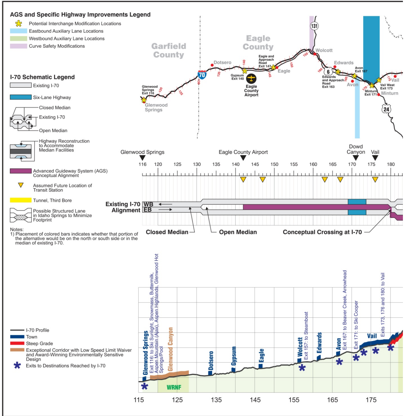
Figure 43. Preferred Alternative – Long Term – Combination 6-Lane Highway with AGS – 55 and 65 mph Options
