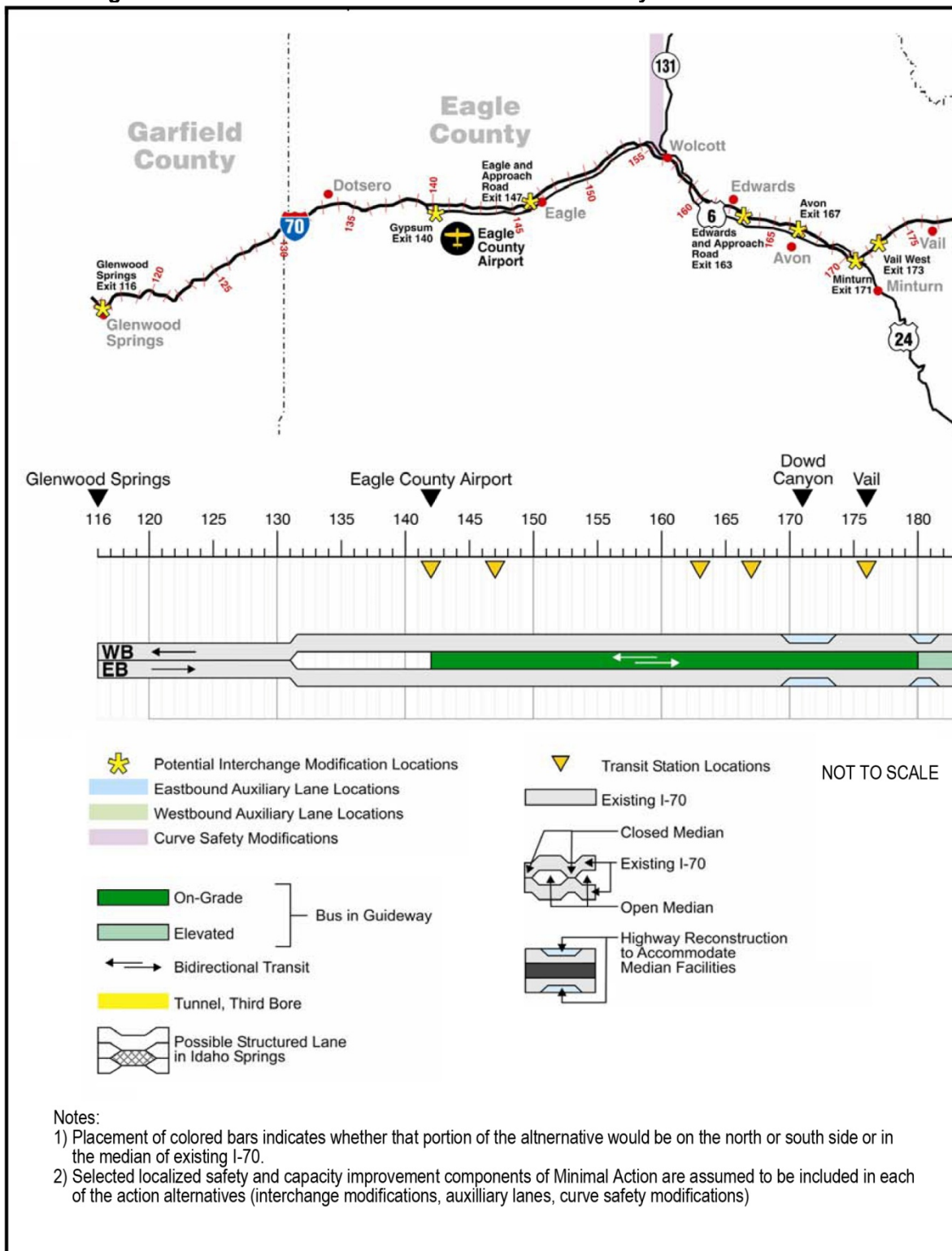
Figure 17. Dual-Mode Bus and Diesel Bus in Guideway Alternative Overview
