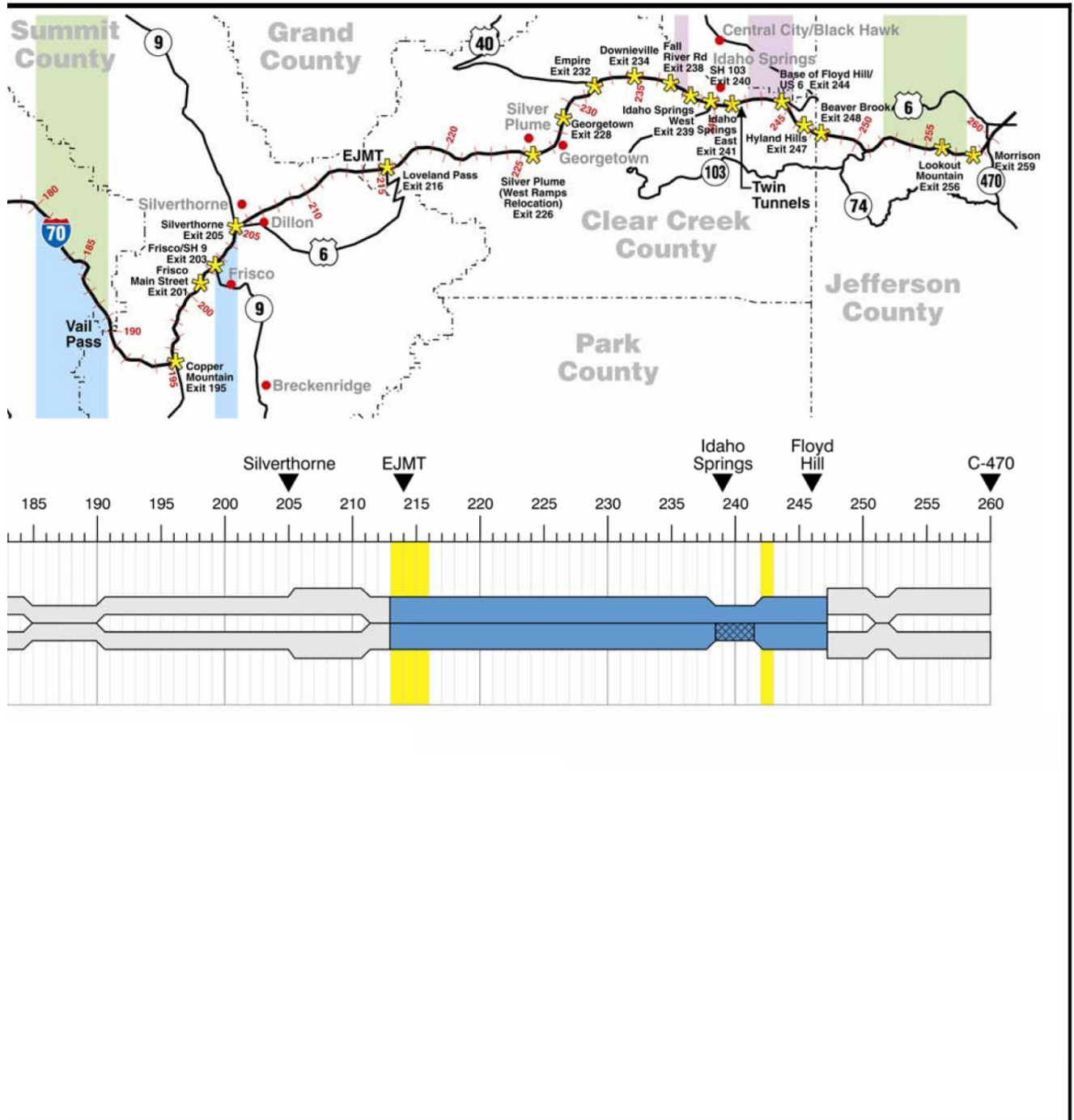
Figure 22. Six-Lane Highway 55 mph Alternative Overview (Continued)
