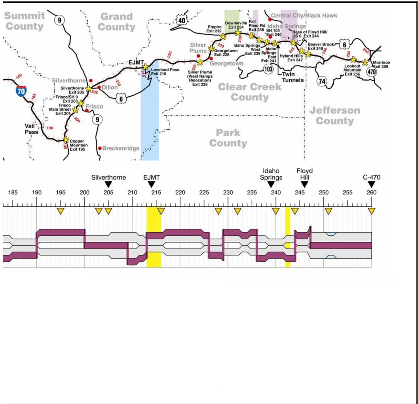
Figure 12. Advanced Guideway System Alternative Overview (Continued)
