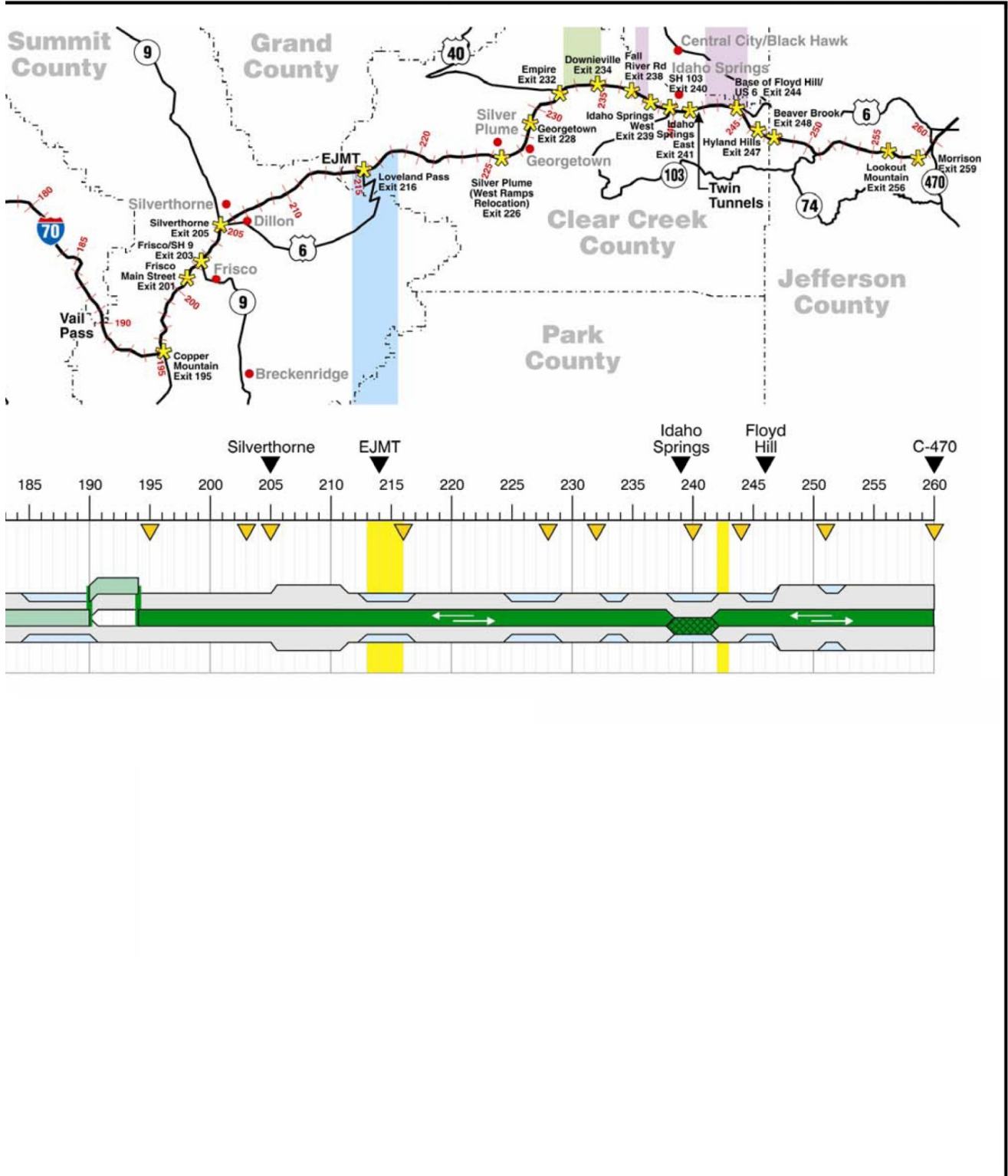
Figure 17. Dual-Mode Bus and Diesel Bus in Guideway Alternative Overview (Continued)
