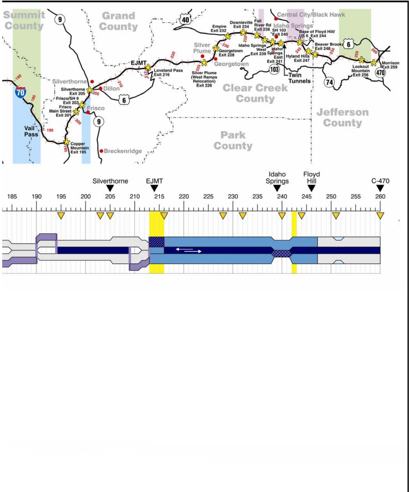
Figure 31. Combination Six-Lane Highway with Rail and Intermountain Connection Alternative Overview (Continued)
