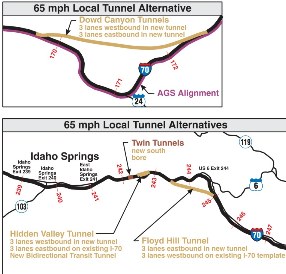
Figure 48. Preferred Alternative (65 mph Option) Tunnel Alternative
