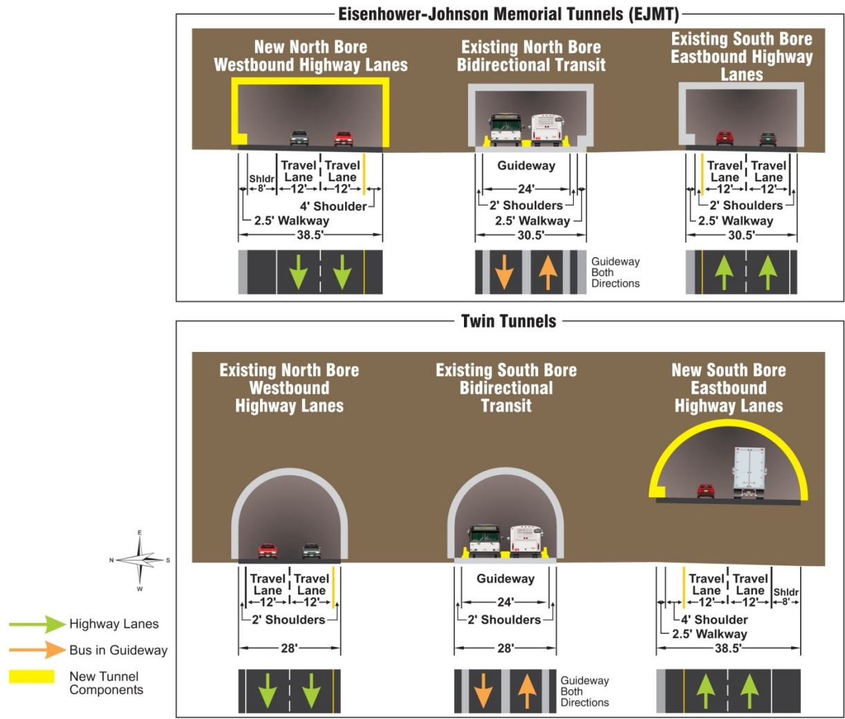
Figure 20. Dual-Mode Bus and Diesel Bus in Guideway Eisenhower-Johnson Memorial Tunnels and Twin Tunnels
