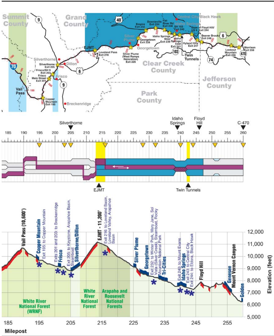
Figure 43. Preferred Alternative – Long Term – Combination 6-Lane Highway with AGS – 55 and 65 mph Options (Continued)
