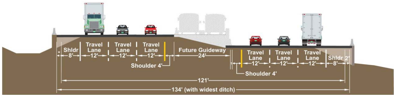
Figure 38. Highway with Bus in Guideway Preservation
