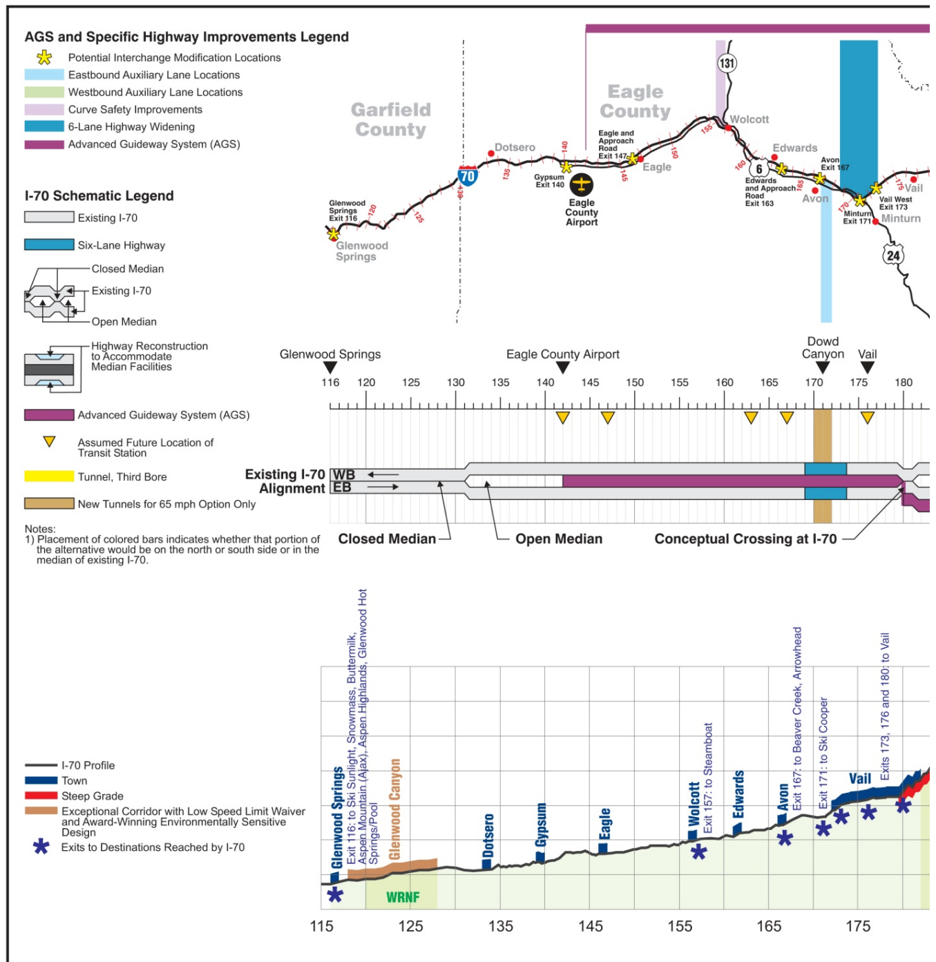
Figure 42. Preferred Alternative Near Term – Advanced Guideway System with Specific Highway Improvements – 55 and 65 mph Options
