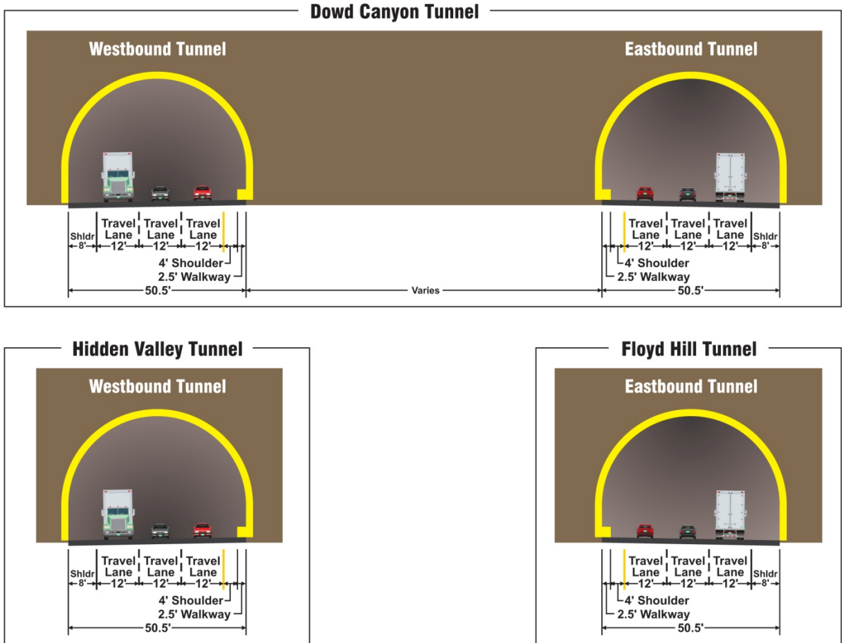
Figure 27. Six-Lane Highway 65 mph Alternative Dowd Canyon Tunnel, Hidden Valley Tunnel, and Floyd Hill Tunnel
