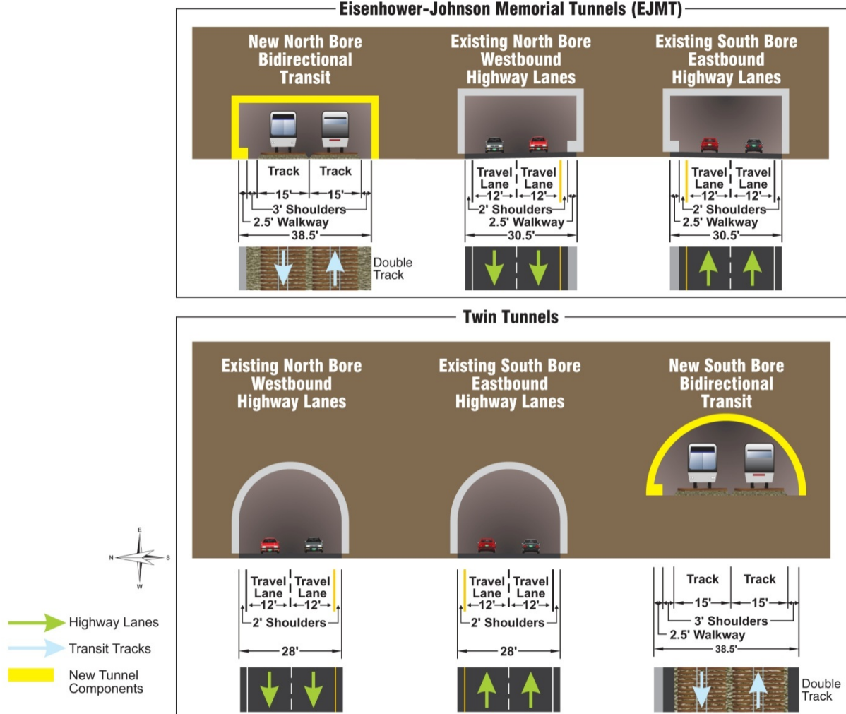
Figure 9. Rail with IMC Cross Section – Eisenhower-Johnson Memorial Tunnels and Twin Tunnels
