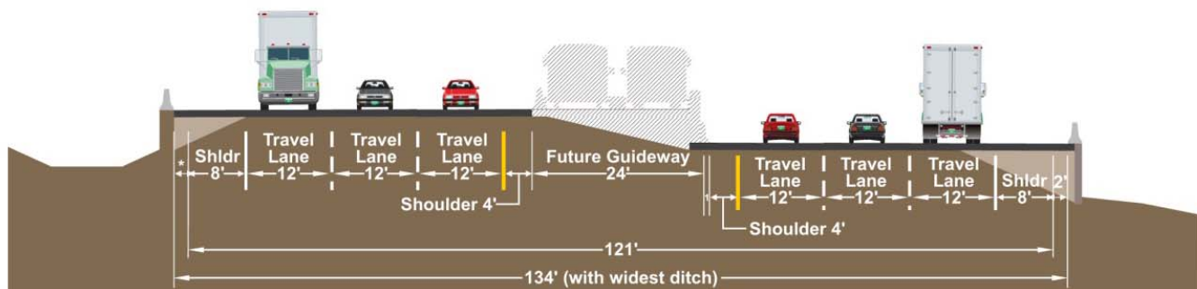
Figure 40. Highway with Bus in Guideway Preservation
