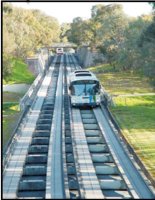
Figure 18. Dual-Mode Bus and Diesel Bus in Guideway Example of Guide Wheels
