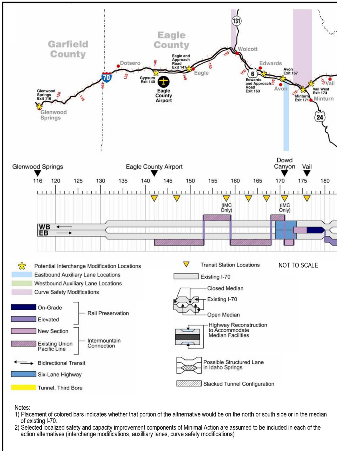
Figure 31. Combination Six-Lane Highway with Rail and Intermountain Connection Alternative Overview
