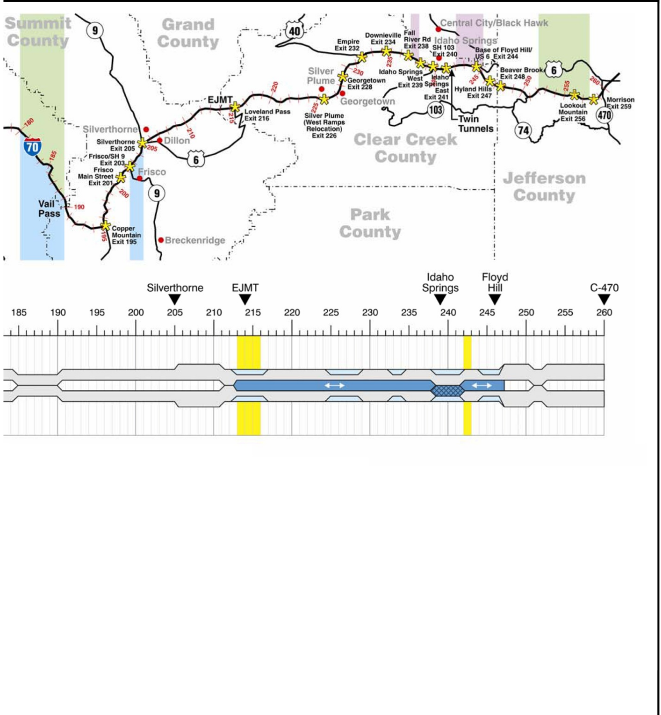
Figure 28. Reversible/High Occupancy Vehicle/High Occupancy Toll Lanes Alternative Overview (Continued)
