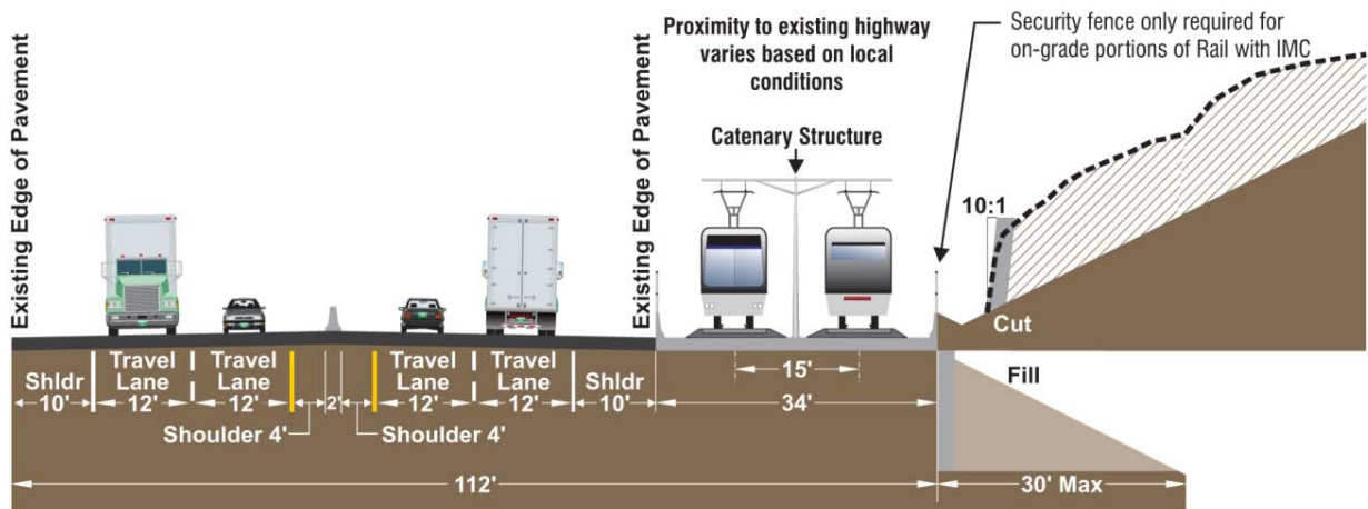
Figure 8. Rail with IMC Cross Section – Typical Configuration
