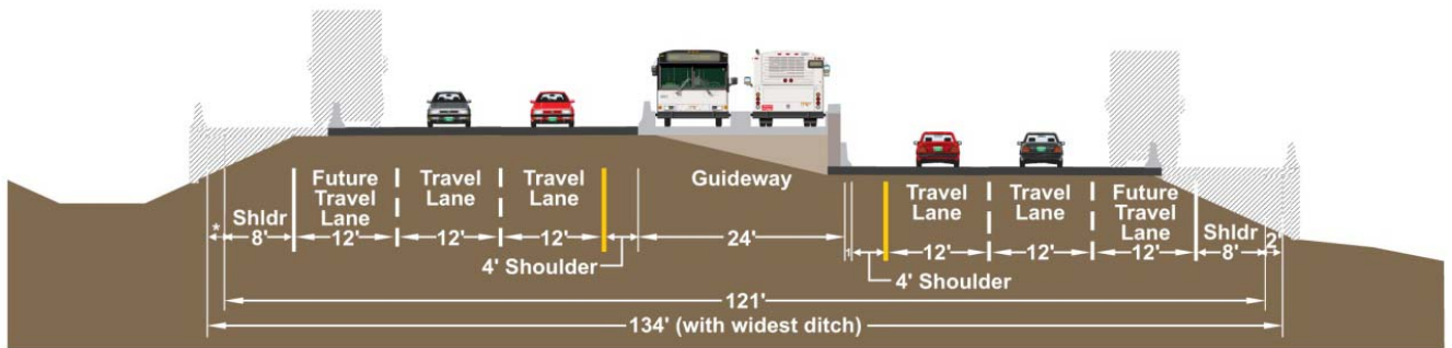
Figure 39. Bus in Guideway with Highway Preservation
