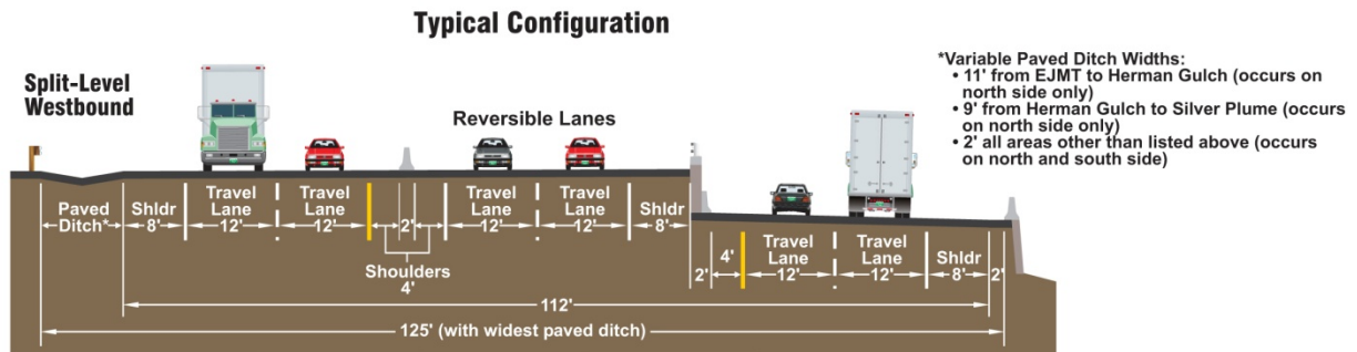
Figure 29. Reversible/High Occupancy Vehicle/High Occupancy Toll Lanes Alternative Typical Configuration and Structured Configuration in Idaho Springs
