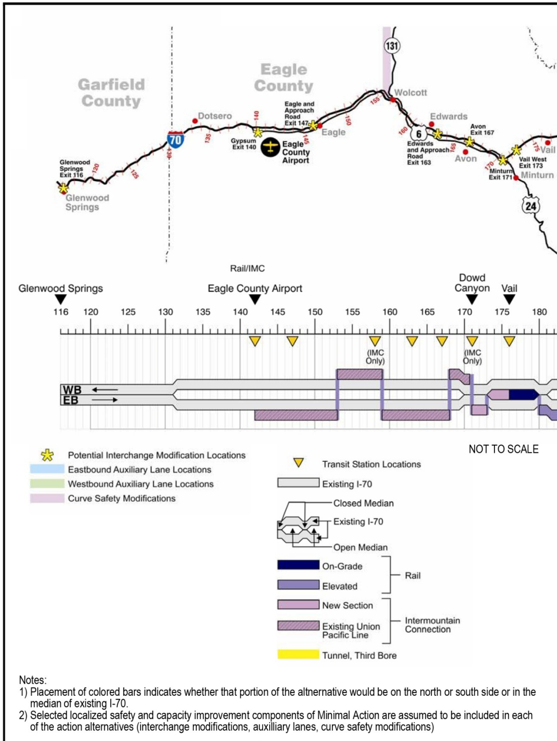
Figure 7. Rail with IMC Alternate Overview
