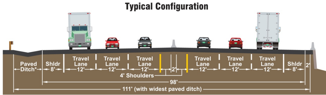
Figure 23. Six-Lane Highway 55 mph Alternative Typical Configuration and Structured Configuration in Idaho Springs
