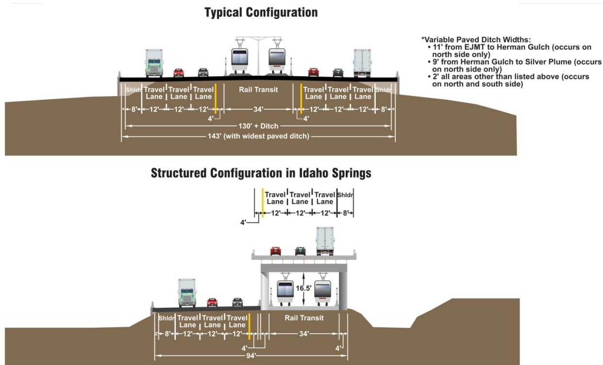
Figure 32. Combination Six-Lane Highway with Rail and Intermountain Connection Alternative Typical Configuration and Structured Configuration in Idaho Springs
