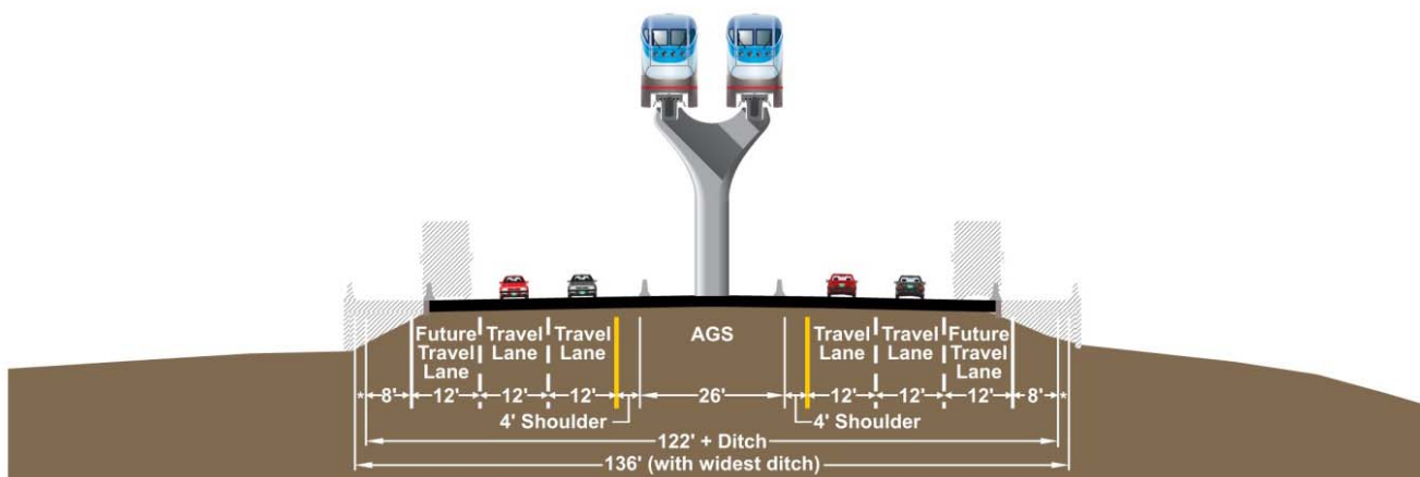
Figure 37. Advanced Guideway System with Highway Preservation
