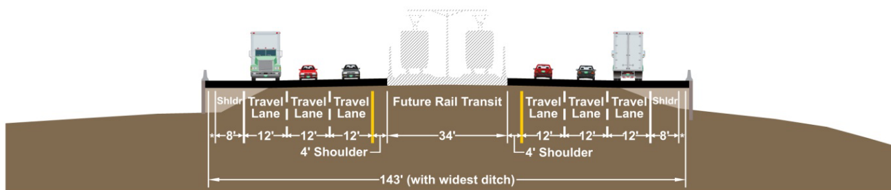
Figure 34. Highway with Rail Preservation
