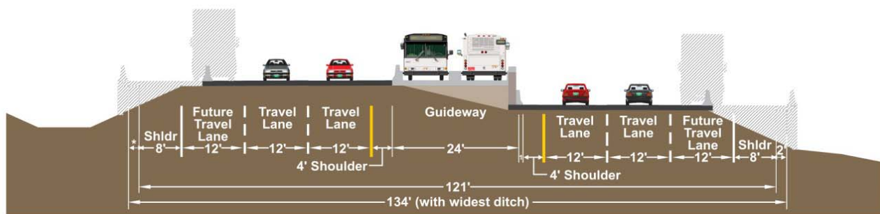
Figure 41. Bus in Guideway with Highway Preservation
