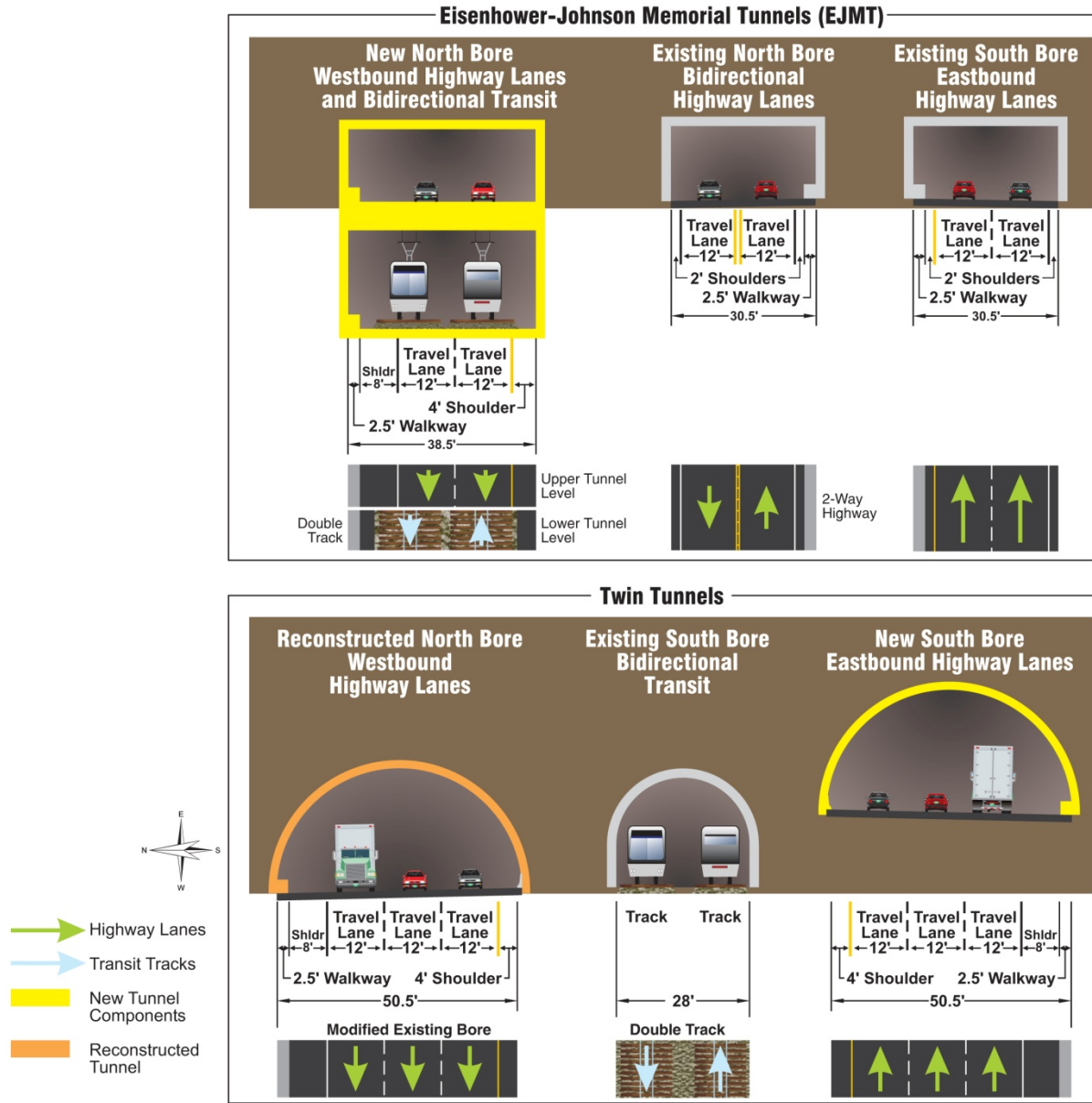
Figure 33. Combination Six-Lane Highway with Rail and Intermountain Connection Alternative Eisenhower-Johnson Memorial Tunnels and Twin Tunnels
