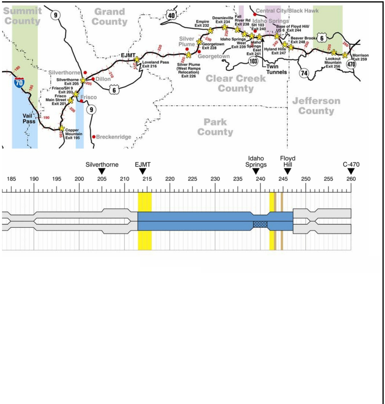
Figure 25. Six-Lane Highway 65 mph Alternative Overview (Continued)
