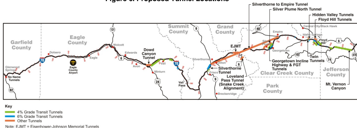
Figure 6. Proposed Tunnel Locations
