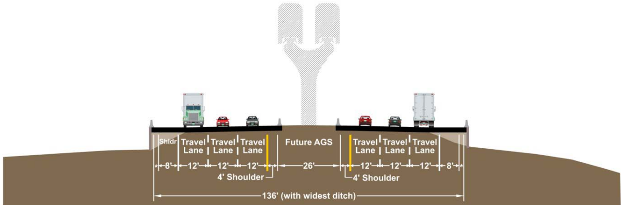
Figure 36. Highway with Advanced Guideway System Preservation
