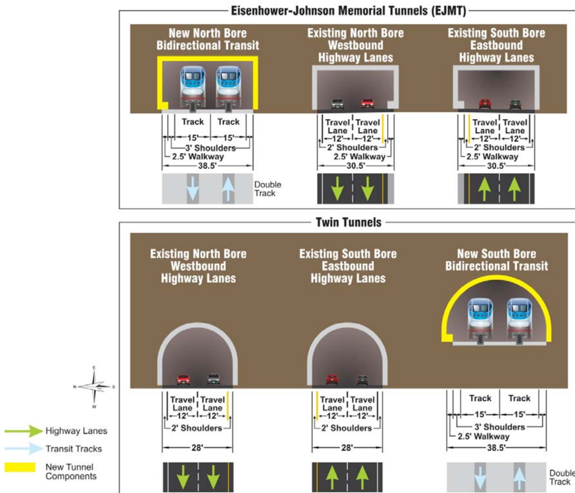
Figure 14. Advanced Guideway System Eisenhower-Johnson Memorial Tunnels and Twin Tunnels
