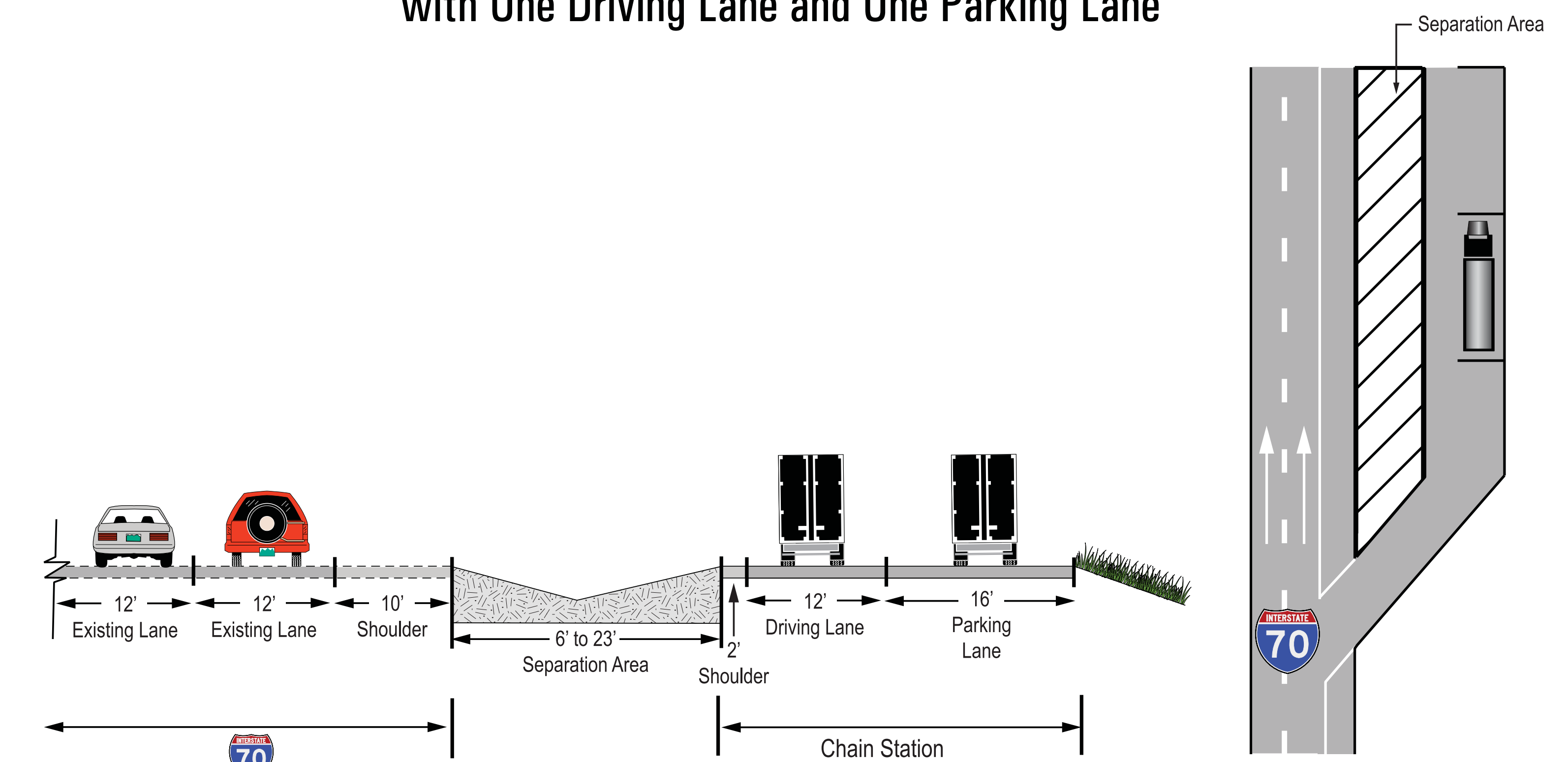
Proposed Typical Chain Station Separated From I-70 with One Driving Lane and One Parking Lane
