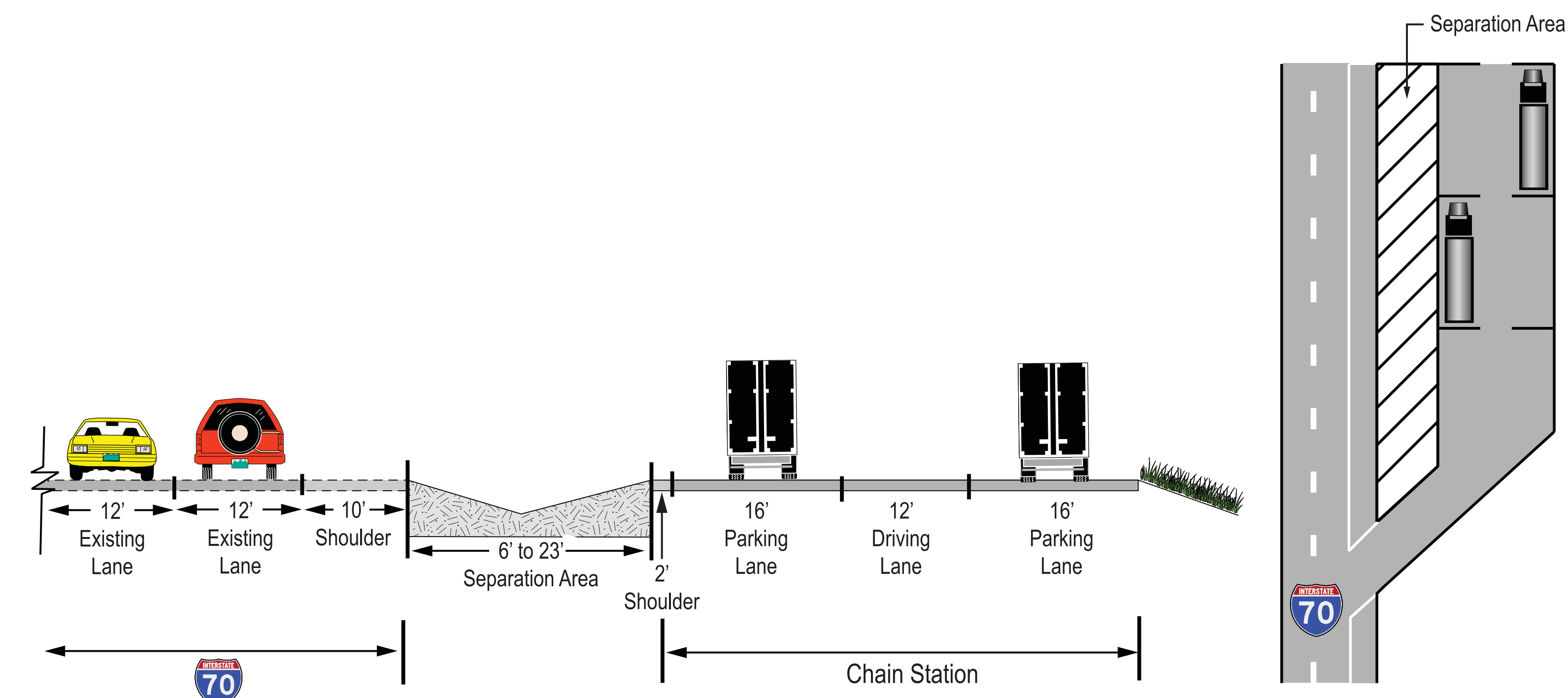
Proposed Typical Chain Station Separated From I-70 with One Driving Lane and Two Parking Lanes
