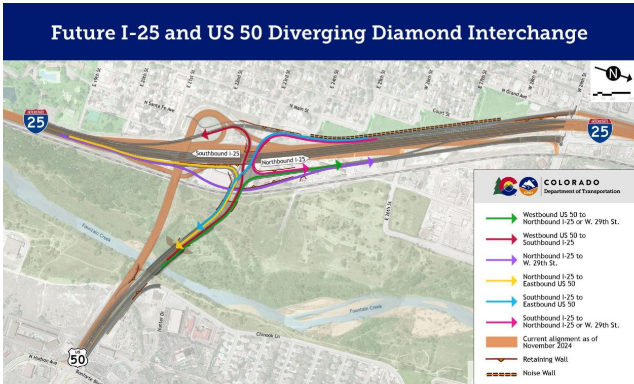
Caption: Rendering of the future I-25 and US 50 Diverging Diamond Interchange in Pueblo. The rendering shows the new interchange configuration and access to US 50, I-25 and W. 29th St.
