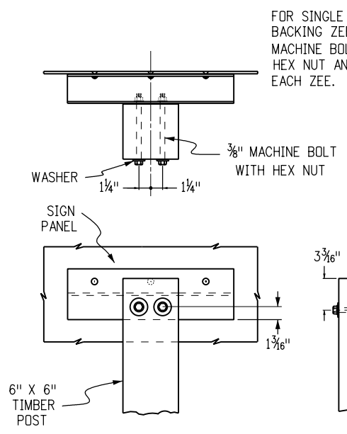
Class II Marker Assembly Installation
