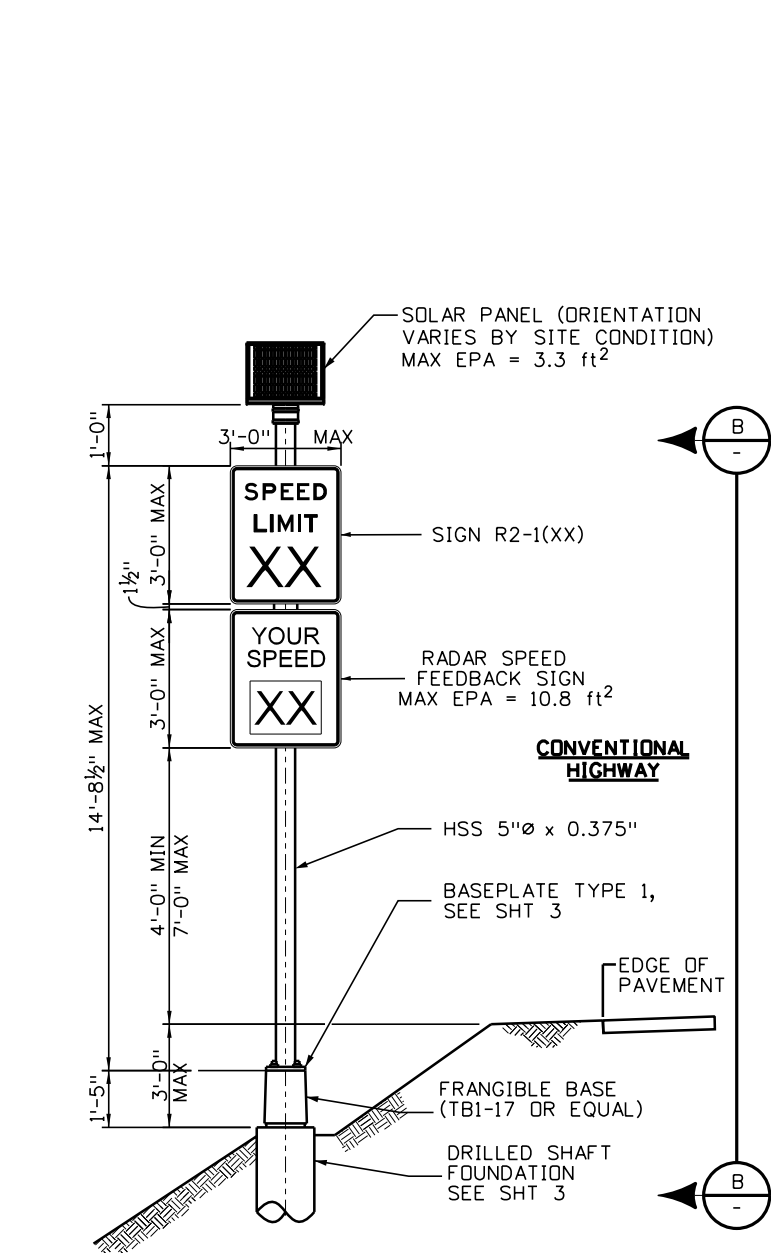
Radar Speed Feedback Sign (Conventional Highway Configuration)
