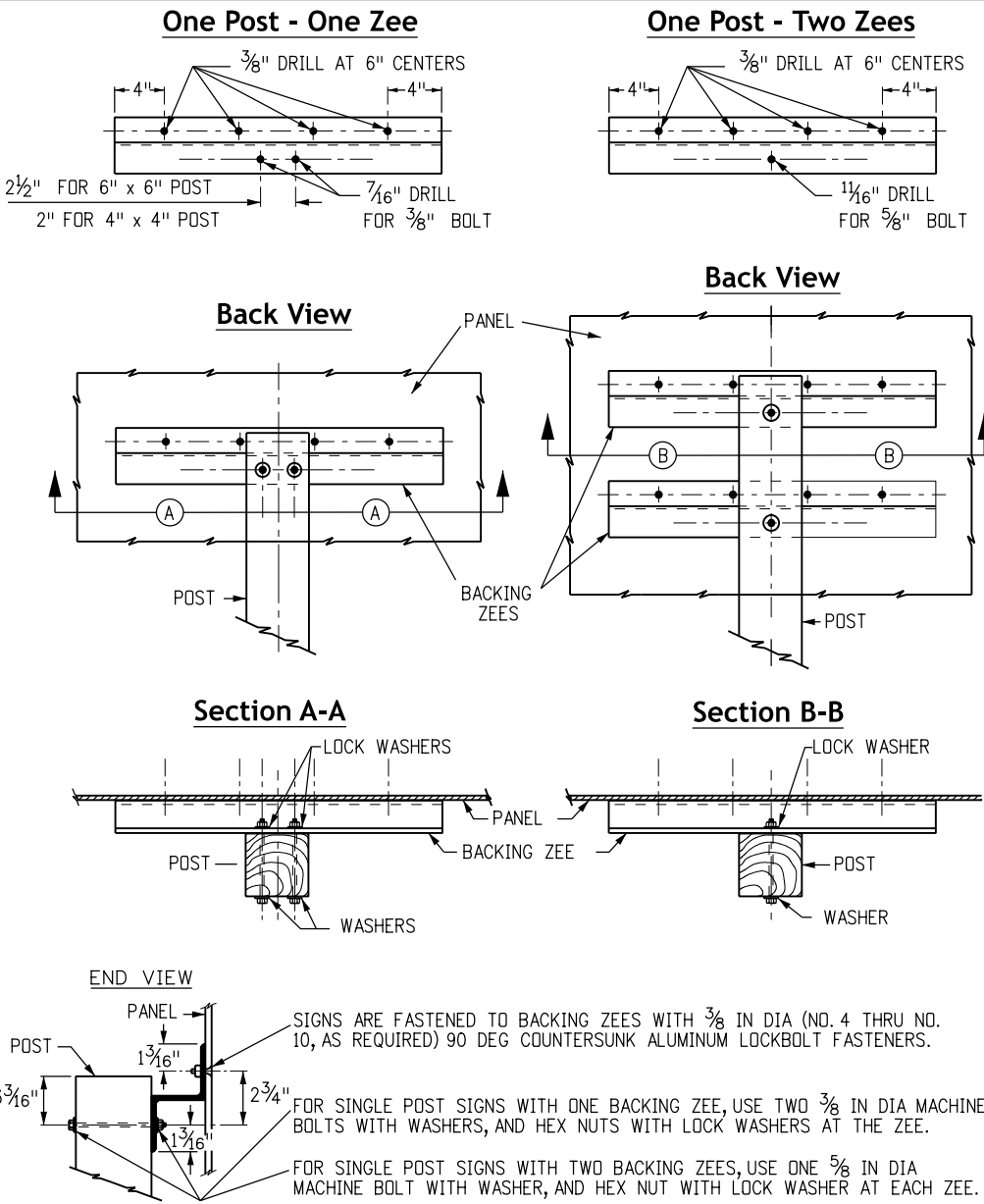
Typical Backing Zees
