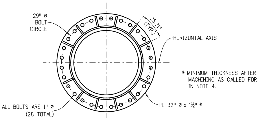
Field Splice Details
