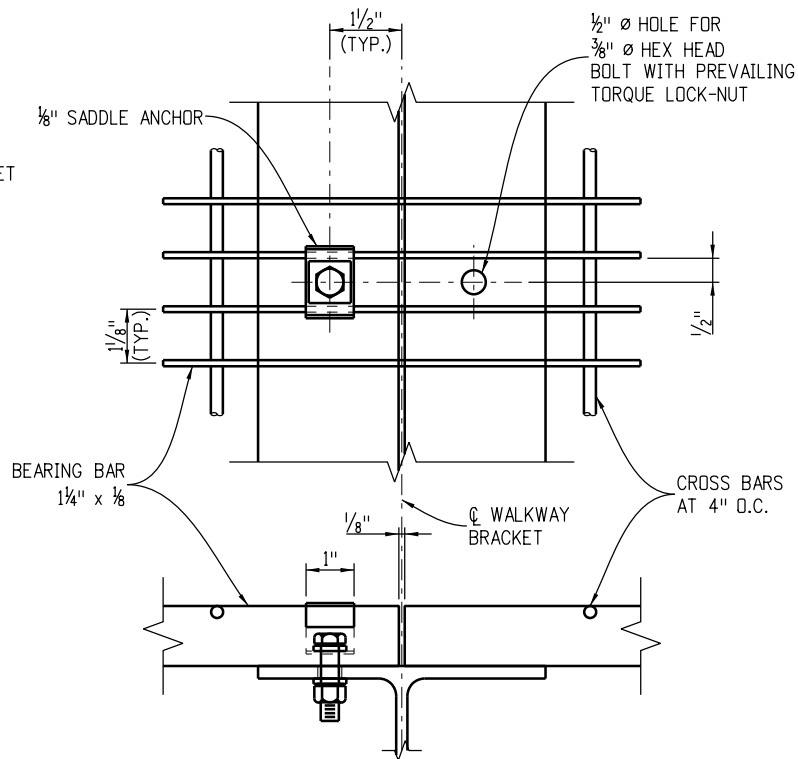
Walkway Details
