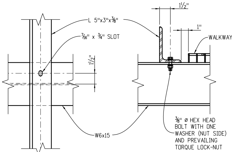
Safety Angle Details
