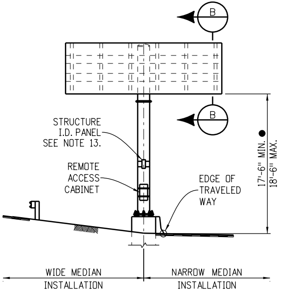
Butterfly Sign (Median Installation) (See Sign X-Section Sheet in Traffic Plans)
