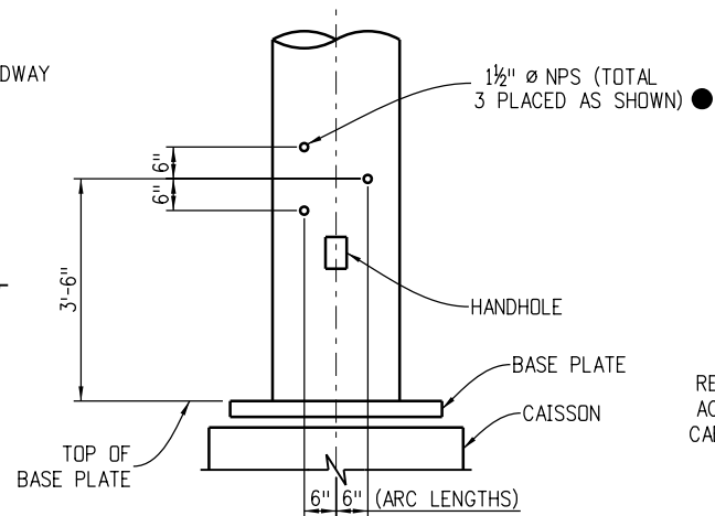
Conduit Penetration Details ● Plug with Recessed Pipe Plugs
