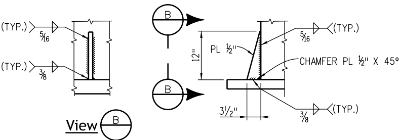
Stiffener Details
