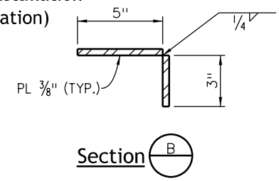
Base Skirt Detail
