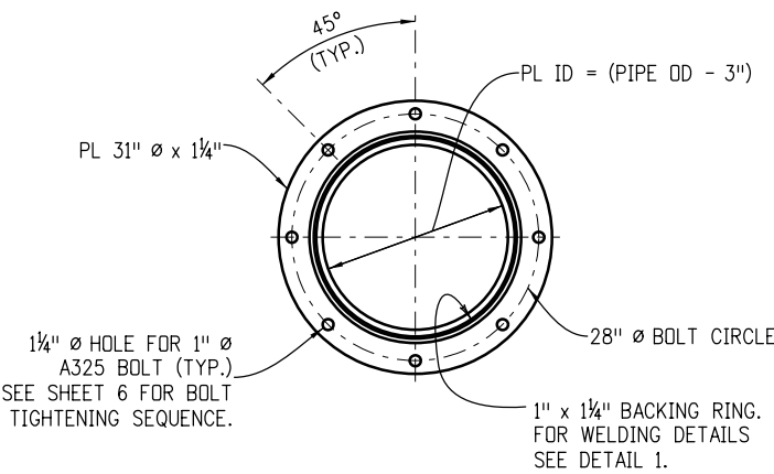
Optional Field Splice 24" Pipe Post
