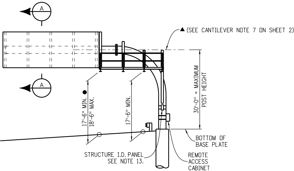
Cantilever Sign
