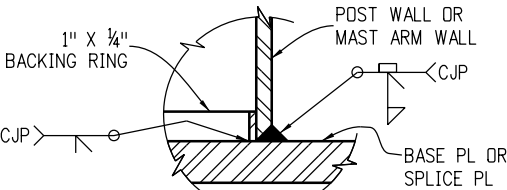
Detail 1
