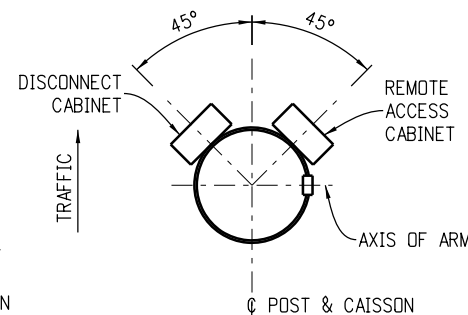
Section C
