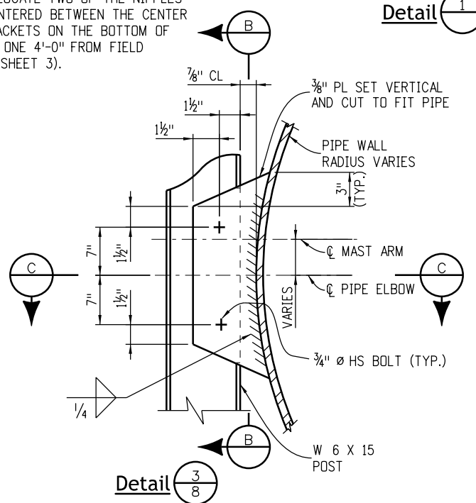
Mounting Bracket on Elbow and Pole
