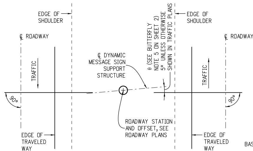
Median Installation Plan
