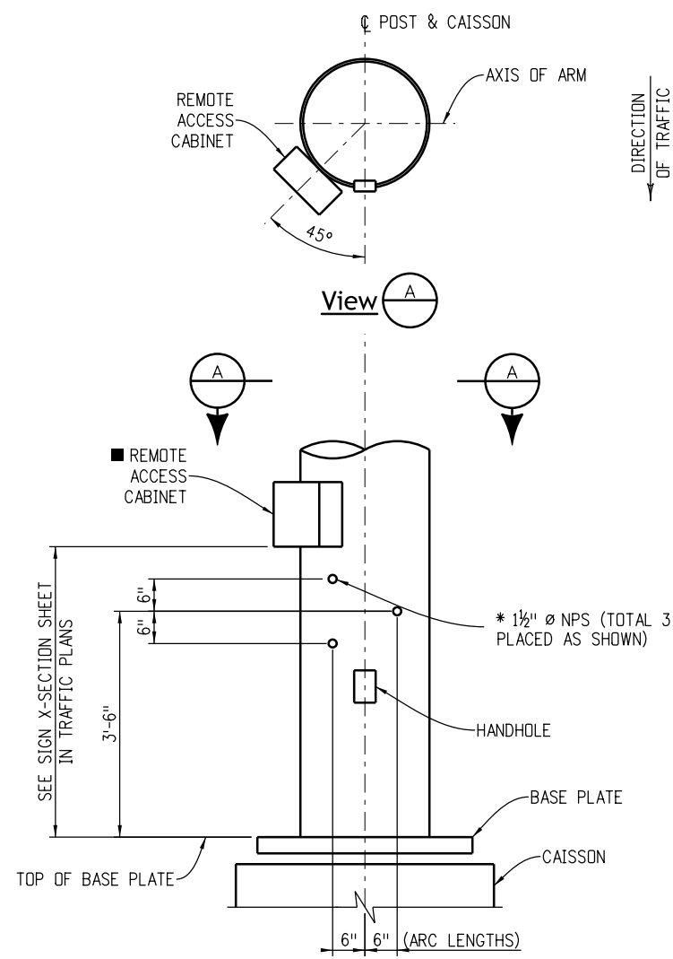
Conduit Penetration Details * Plug with recessed pipe plugs. ■ Disconnect cabinet for the power supply shall be located outside of the clear-zone.
