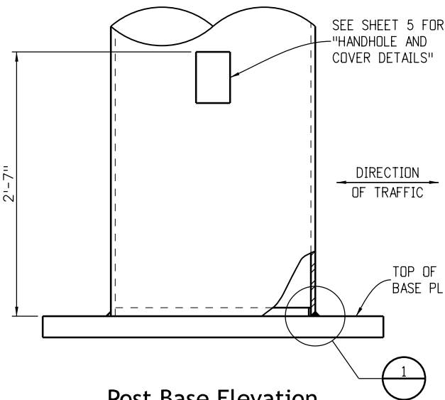
Post Base Elevation
