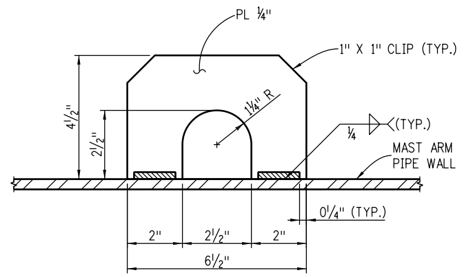
Lifting Eye Detail
