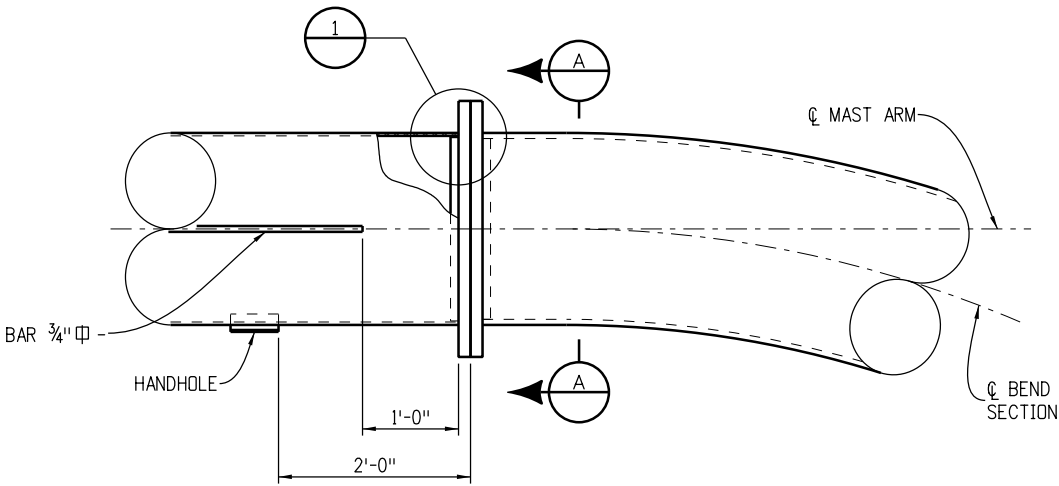
Field Splice
