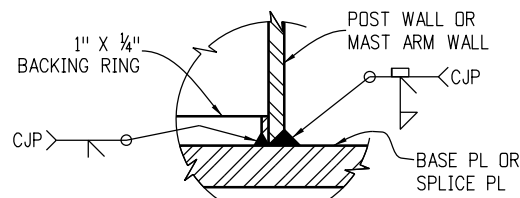
Detail 1
