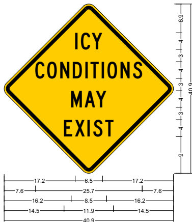
30W8-49; 30.0" across sides 1.9" Radius, 0.8" Border, 0.5" Indent, Black on Yellow;
