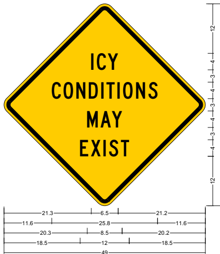
36W8-49; 36.0" across sides 2.3" Radius, 0.9" Border, 0.6" Indent, Black on Yellow;
