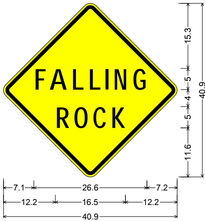
30.0" across sides 1.9" Radius, 0.8" Border, 0.5" Indent, Black on Yellow; "FALLING" D; "ROCK" D; Table of letter and object lefts.
