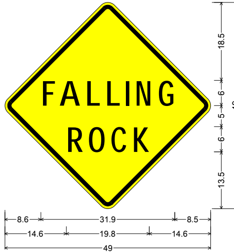
36.0" across sides 2.3" Radius, 0.9" Border, 0.6" Indent, Black on Yellow; "FALLING" D; "ROCK" D; Table of letter and object lefts.
