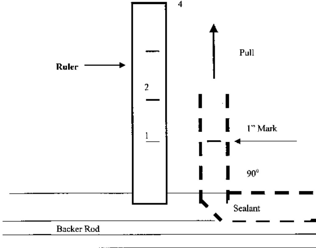
FIGURE 67-4 Pull Initiation
